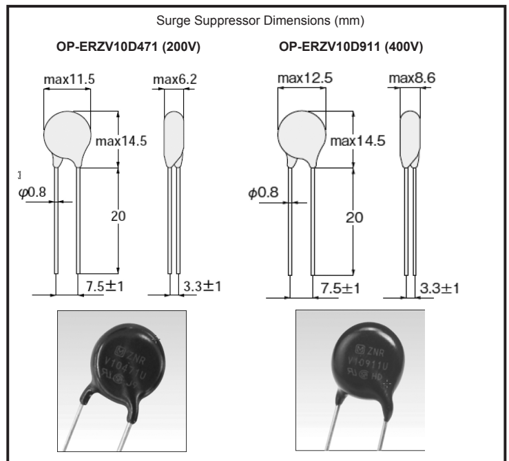
Fig. 1.16B Surge Suppressor
