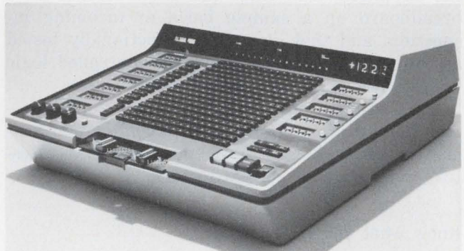
A small, bench-top tester , the Alma 480B, is programmed from the front panel by a pushbutton array and thumbwheel switches. Most other bench-top testers use personality cards to match the tester to the device.
