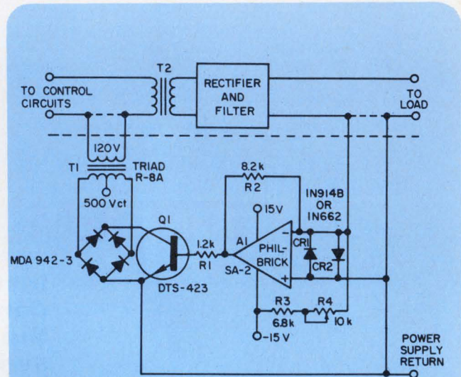
Output current above 1.5 mA causes op amp A_1 to turn transistor Q_1 off, creating a high impedance at transformer T_1 's secondary. This high impedance is reflected into T_1 's primary, limiting further increases in load current.
