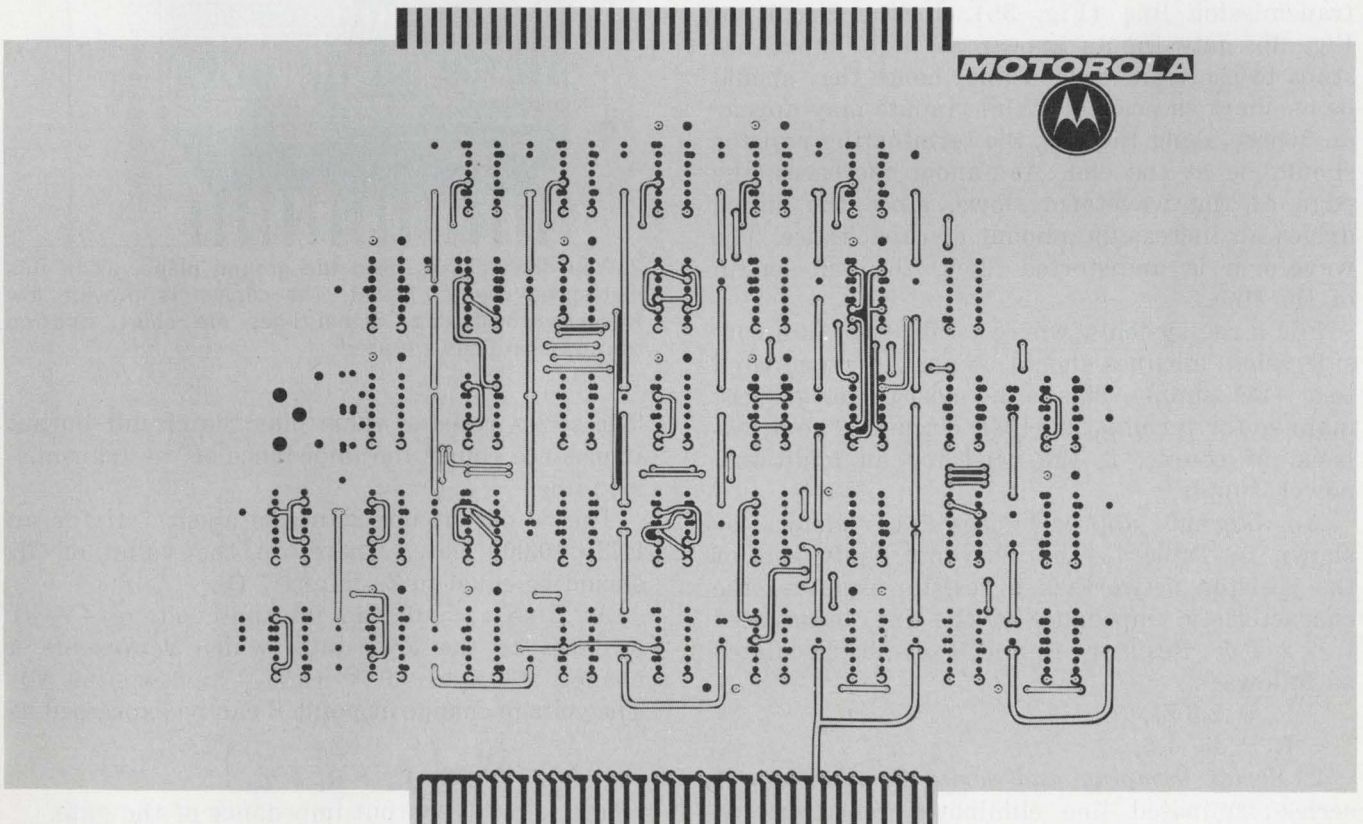
1. A MECL 10,000 PC board with a ground plane. The board provides a constant characteristic impedance and low inductance path for ground currents. The ground
