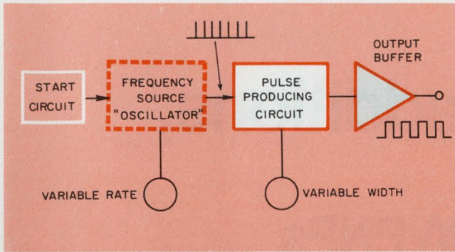
1. Pulses are initially generated by a variable frequency oscillator. These pulses then trigger a monostable multivibrator with adjustable time constant which determines the output pulse width. Output buffer provides additional amplification.
