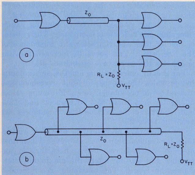
3. Parallel-terminated lines can have lumped (a) or distributed (b) fanouts. A termination voltage, V_{TT} , is required to prevent excessive termination-resistor power.
