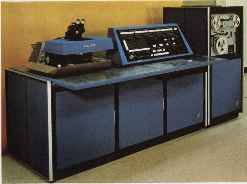
An example of the newer machines is Western Digital's Spartan 770 MOS/LSI tester. It uses a bipolar, microprogrammable RAM instead of the ubiquitous minicomputer of other systems.
