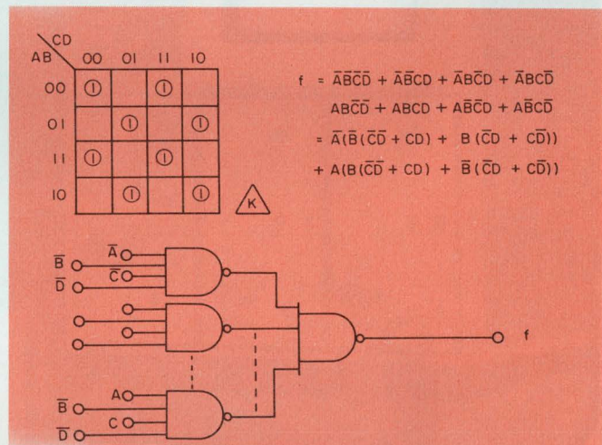
6. Karnaugh reduction in this example results in a circuit that requires five DIPs and 32 inputs. Contrast this with the Ring-map reduction in Fig. 7.
