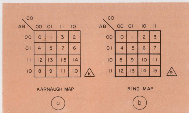
1. The standard Karnaugh map representation (a) of a four-variable logic function is modified (b) to form the Ring map. Boxes are numbered for identification.
