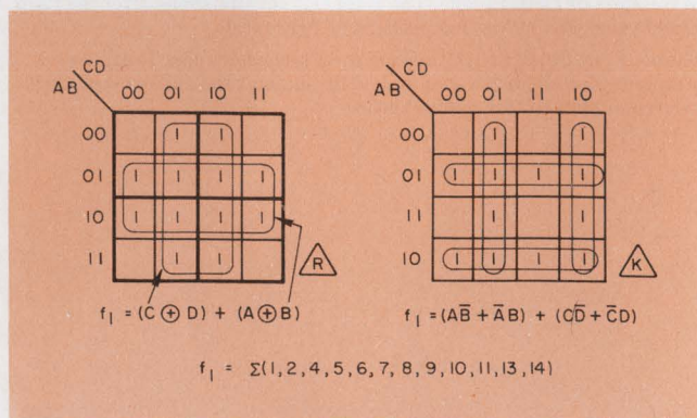
2. EXCLUSIVE-OR functions contained in f_1 are spotted immediately on the Ring map, but the Boolean equation for f_1 that is derived from the Karnaugh map must be manipulated to minimize the function.
