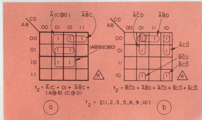
3. Functions containing mixed terms are easily handled by the Ring map (a). The standard Karnaugh procedure is shown in (b).
