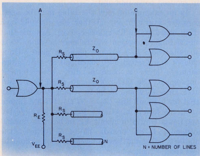
5. With N lines, N loads are obtained on a series-terminated line. Resistor R_E must be less than a maximum value fixed by the number of lines and Z_0 to prevent the output transistor from turning off during switching.
