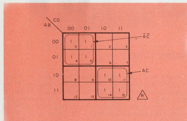
4. EXCLUSIVE-ORs formed from row and column variables are not readily detected, since the implicants do not cross Ring-map boundaries.
