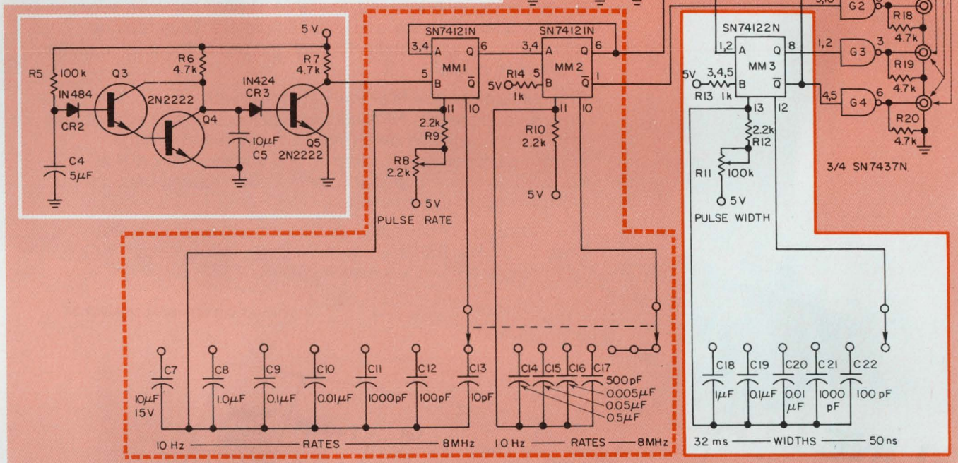
2. One-shots MM_1 and MM_2 act as a variable rate generator, and retriggerable one-shot MM_3 produces variable
