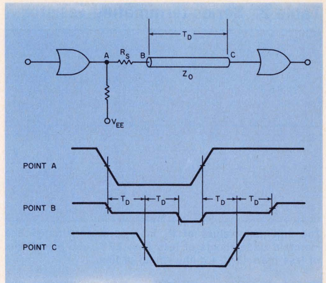
4. Series-terminated lines don't need the extra power supply. But you can't have distributed fanouts because of the half-voltage waveform on the line (waveform B).
