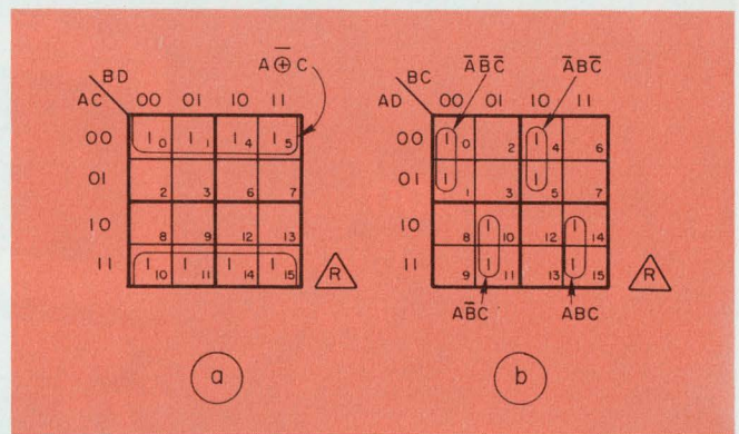
5. To detect EXCLUSIVE-ORs that don't cross boundaries, the map of Fig. 4 is redrawn by combining row and column variables. A is combined with C in "a" and with D in "b."
