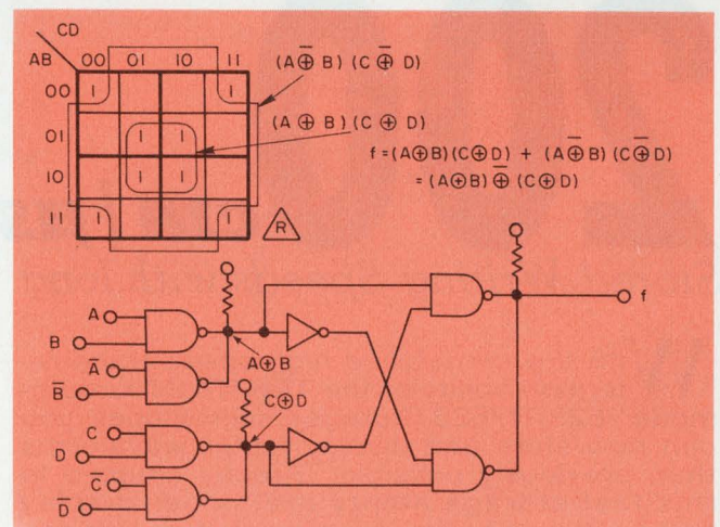
7. Resulting Ring-map circuit needs only two DIPs with eight inputs. A considerable cost savings is realized with the Ring map.
