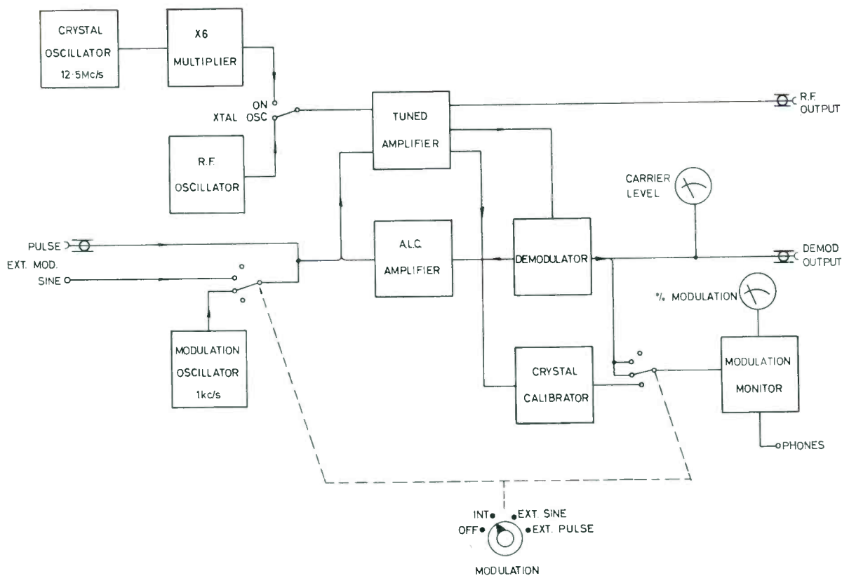
Fig. 1. Block diagram of TF 801D/5M1
