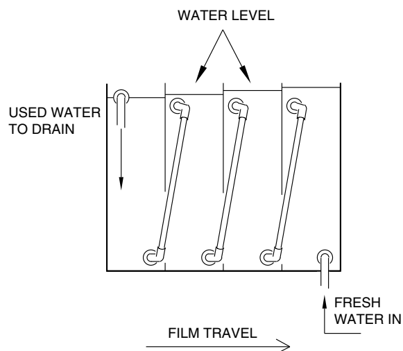
Figure 9-5 Four-Stage Countercurrent Wash
