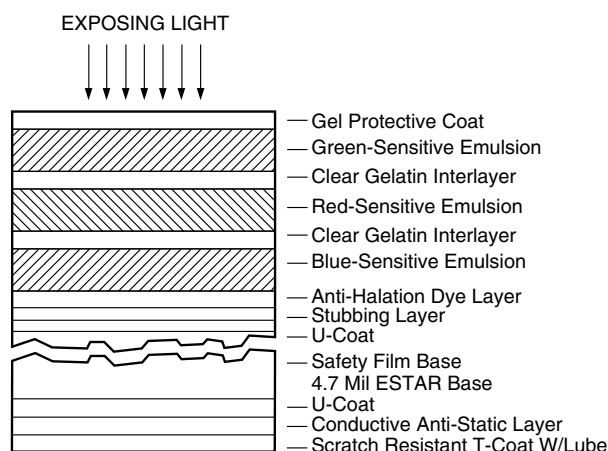
Figure 9-1 Cross Section of Unprocessed Color Print Films
