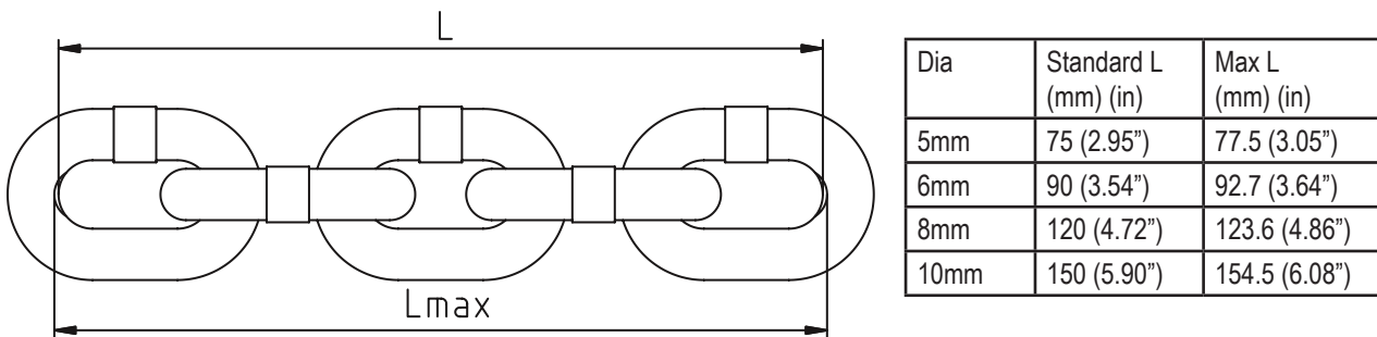
Load Chain - Five link length
