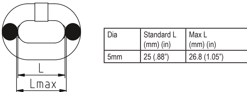
Hand Chain - One link length
