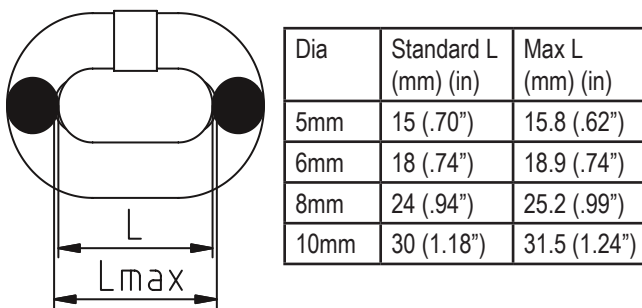
Load Chain - One link length
