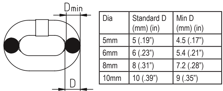
Load Chain - Diameter
