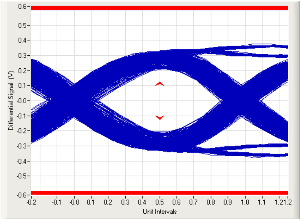
Figure 4. Gen2 -3.5dB Worst transition signal eye
