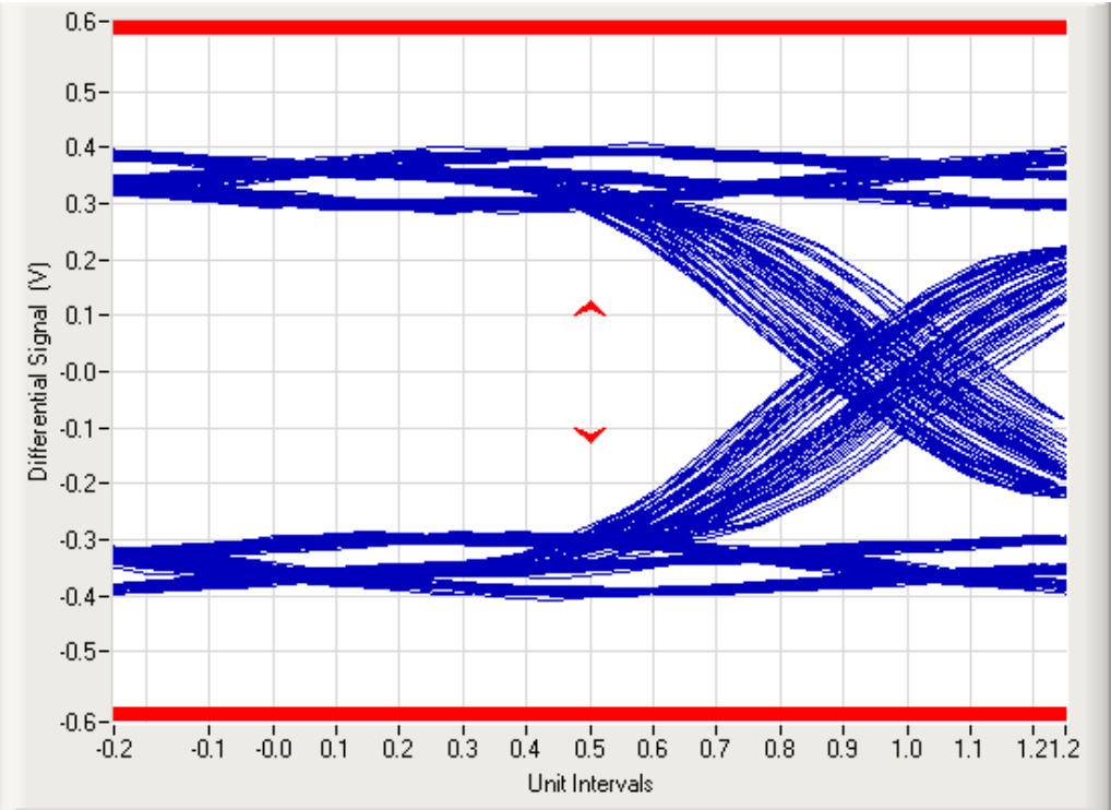
Figure 3. Gen2 TX -3.5dB Worst nontransition signal eye
