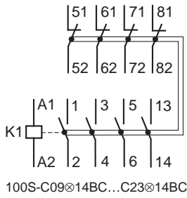
Figure 8 - Safety Contactors with 3 Main Contacts and Bifurcated Front-mount Auxiliary Contacts
