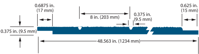
LP SMARTSIDE 120 SERIES CEDAR PANEL 8 IN. O.C.
