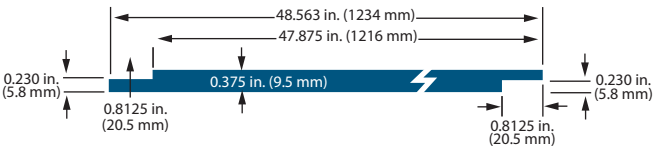
LP SMARTSIDE 76 SERIES PANEL (NO GROOVE)
