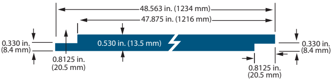
LP SMARTSIDE 190 SERIES PANEL (NO GROOVE)
