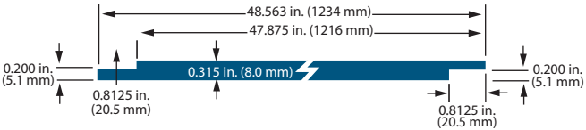
LP SMARTSIDE 38 SERIES PANEL (NO GROOVE)
