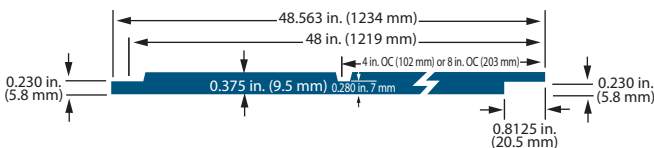
LP SMARTSIDE 76 SERIES PANEL 4 IN. & 8 IN. O.C.
