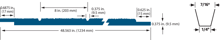
LP® SMARTSIDE® CEDAR 76 SERIES PREFINISHED 8 IN. O.C. PANEL SIDING
