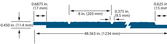
LP SMARTSIDE 120 SERIES CEDAR PANEL 8 IN. O.C.
