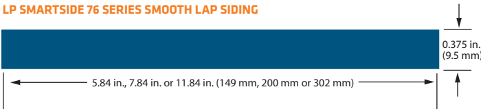
LP SMARTSIDE 76 SERIES SMOOTH LAP SIDING
