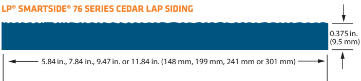
LP® SMARTSIDE® 76 SERIES CEDAR LAP SIDING
