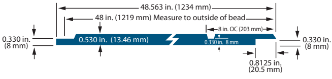
LP SMARTSIDE 190 SERIES PANEL 8 IN. O.C.
