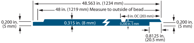
LP SMARTSIDE 38 SERIES PANEL 8 IN. O.C.
