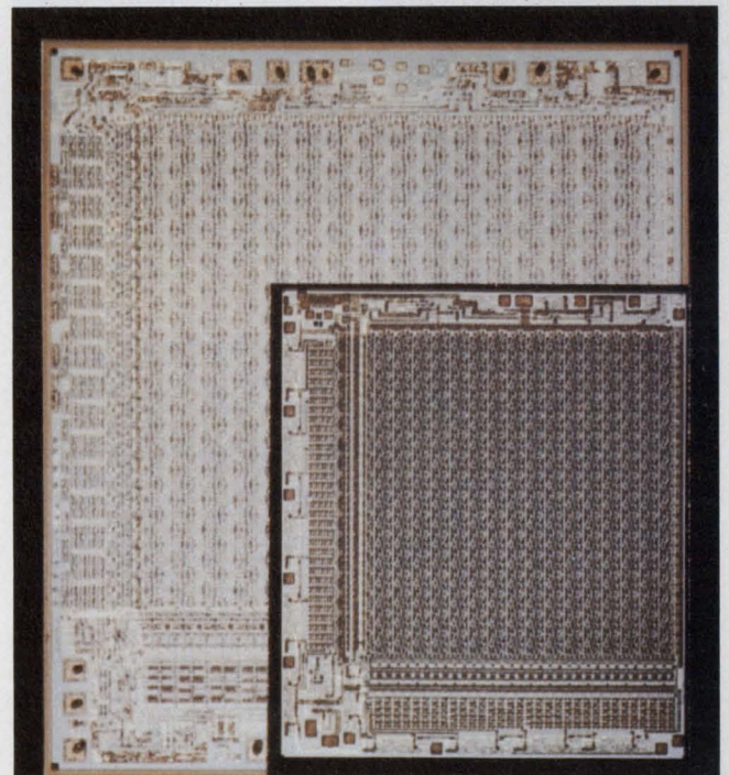
The size of the die directly affects the cost of a semi memory. The original design of this 1024-bit memory from Signetics is shown in the background; it requires 25,000 sq mil of silicon. The present design, shown in the foreground, is only 14,500 sq mil. Data sheets often indicate the die size.
