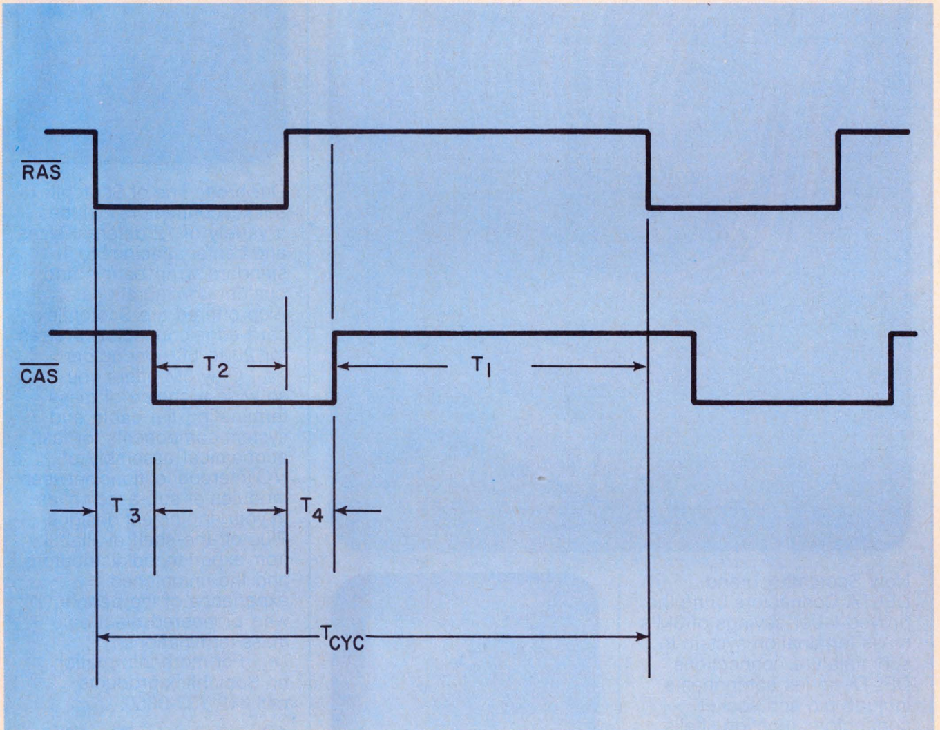
1. Timing waveforms for a 4-k RAM read/write cycle show relationships needed to calculate the ac component of I_{DD} .
