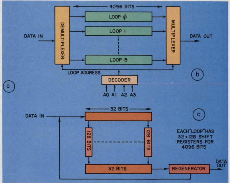
loop 4096-bits long. Four address pins describe which loop accepts or delivers data (b). Each loop is actually an arrangement of serial-parallel-serial shift registers, in a format of 32 \times 128 \times 32 bits (c).
