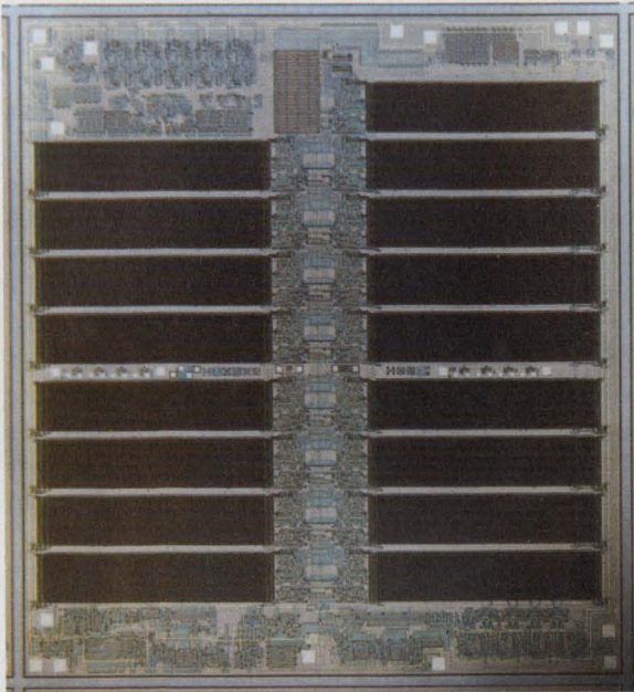
The advantage of CCD memories over dynamic RAMs is that about 70% of the chip area is used for storage, while dynamic RAMs use less than half. TI's CCD, the TMS-3064 (a), is organized as an array of 16 shift-register loops, each
