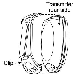
Figure 3 - Clip Attachment
