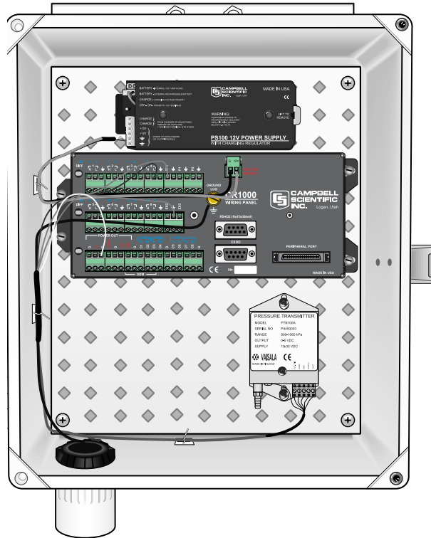
FIGURE 1. CS105 Mounted on the Backplate of an ENC12/14 Enclosure, and Connected to a CR1000 Datalogger
