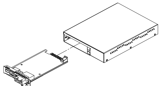
Figure 2-3 Converting FRM220 line card for stand-alone use
