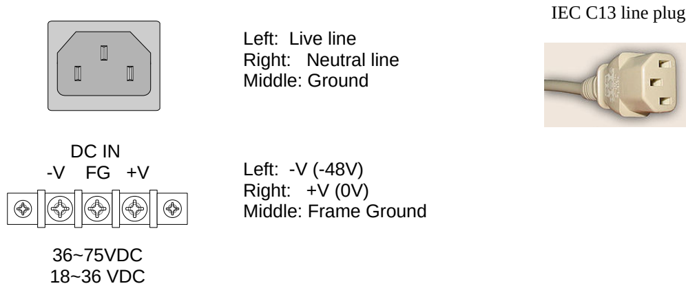
Figure 2-4 IEC (AC) & terminal block (DC) power connector pin assignment
