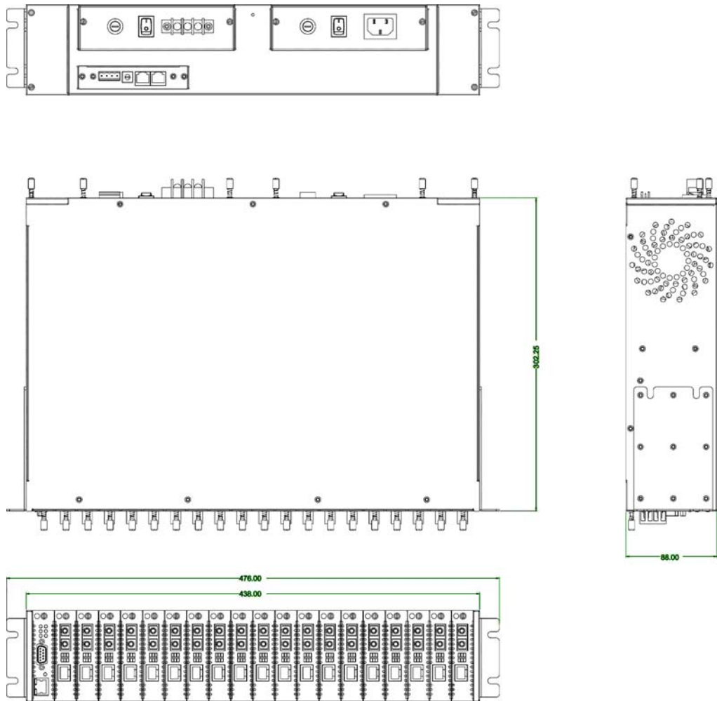
Figure 1-3 Chassis Dimensions, in millimeters
