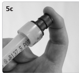
ProPEX Fitting Inserted into 1/2" Uponor PEX Tubing. Make the Fitting with a ProPEX Hand Expander Tool.
