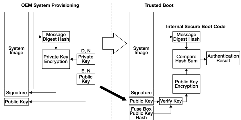
Figure 2: Code Signing and Signature Validation
