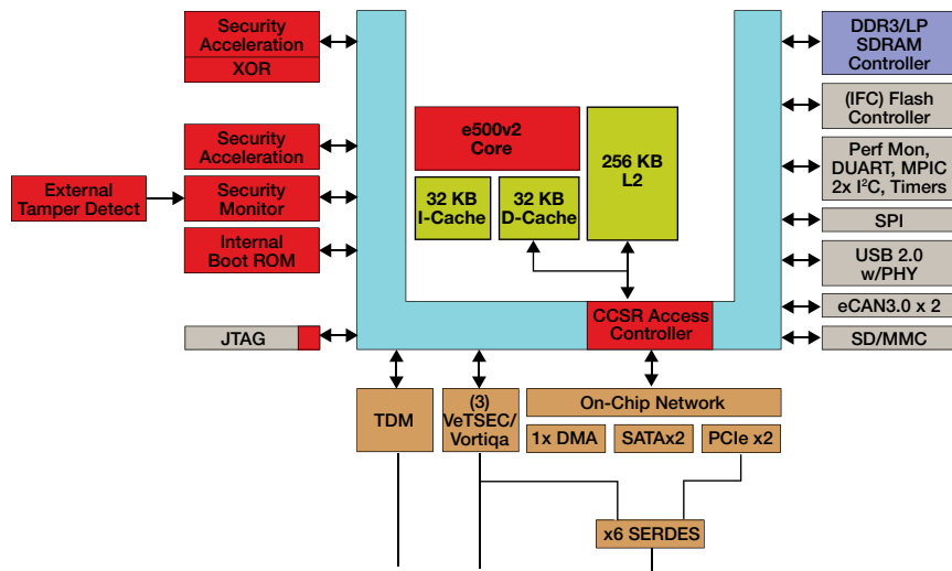
Figure 1: P1010 with the QorIQ Platform's Trust Architecture
