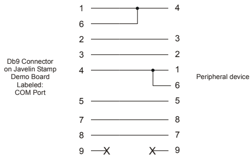
Figure 4.10 shows what's inside the null modem adaptor. Note that it re-routes transmit lines to receive pins and visa-versa.
