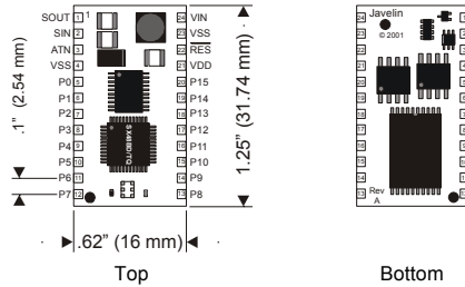
Figure 2.2 Javelin Stamp Mechanical Drawings and Pin Map
