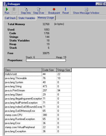
Figure 2.10 IDE Debugger
