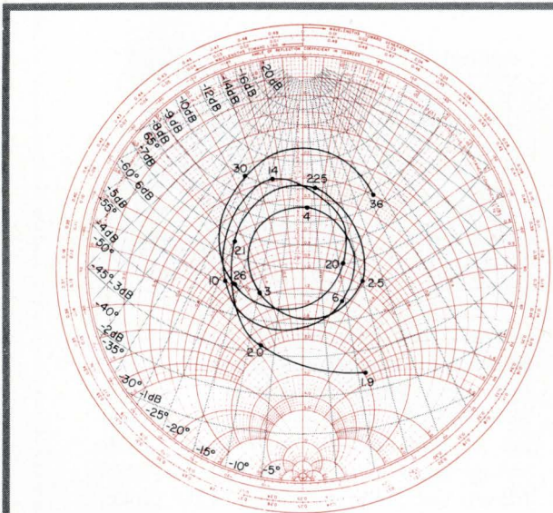
A graph of the input impedance of a 2—32 MHz bandpass filter operating into a mismatched load is shown above. The measurements were made using the test setup described in this article.
