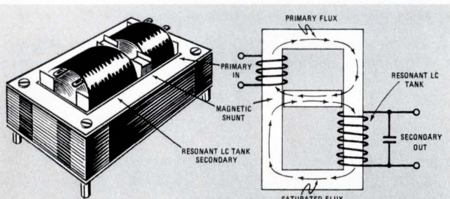
THE FERRORESONANT POWER TRANSFORMER WITH ITS TANK CAPACITOR STABILIZES A d-c OUTPUT WITH A MINIMUM OF FUSS AND BOTHER; AND A MAXIMUM OF RELIABILITY
