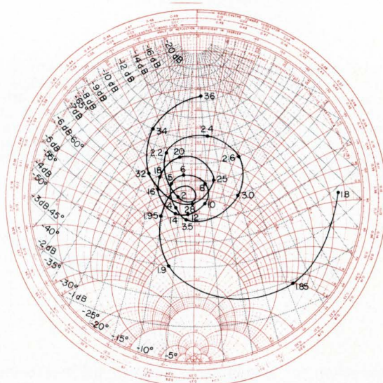
The Smith chart above shows the input impedance when the same 2—32 MHz bandpass filter feeds a transistor amplifier. For this case the input VSWR is also shown. The VSWR is readily derived from the Smith chart by swinging a
