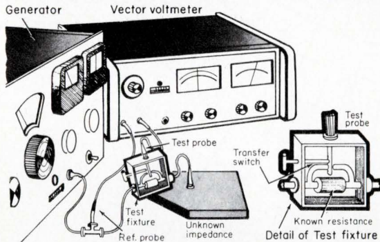
Fig. 1. The test setup shows the simple fixture needed to make impedance measurements. It consists of a known resistance, R , mounted with a transfer switch. To make a measurement, first connect the test probe to the reference probe and set the voltmeter to reference 0 dB, 0 angle. Then read the voltage and angle on the load side of R and plot these on the Smith chart. The unknown impedance can then be read directly off the Smith chart.
