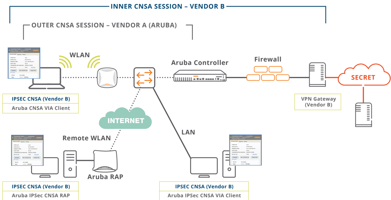
Example Classified Access Architecture with Aruba CNSA Cryptography.
