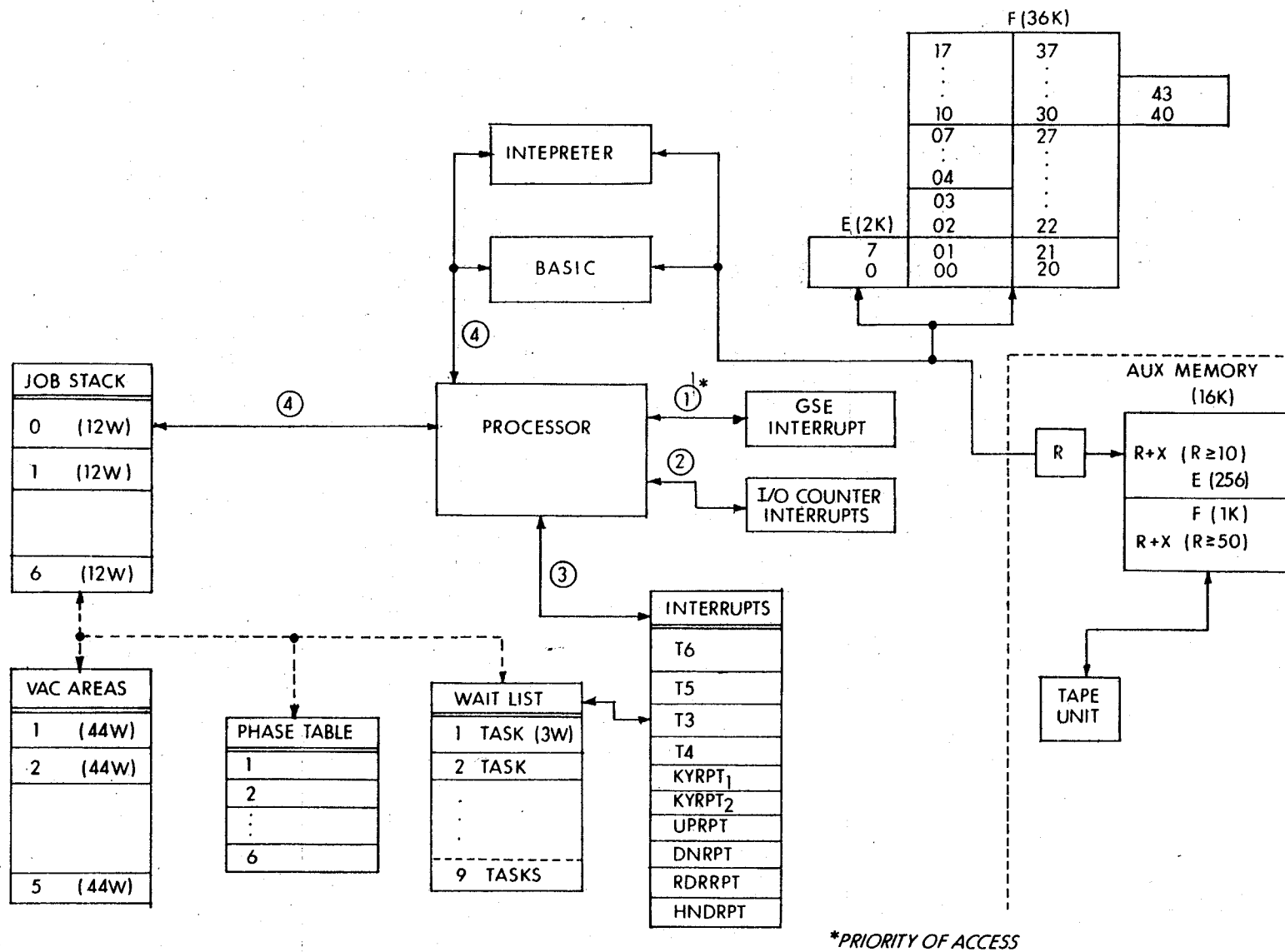
Fig. 1 AGC - Aux Memory.
