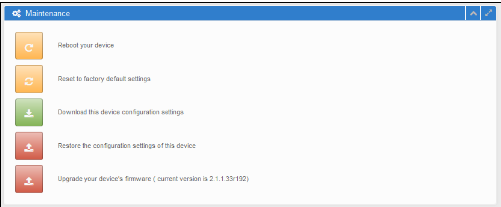
Figure 18: Maintenance
