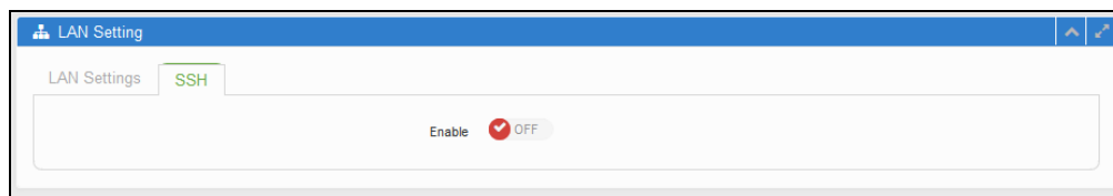
Figure 11: SSH Setting
