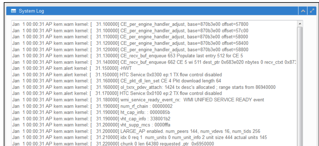
Figure 15: System Log
