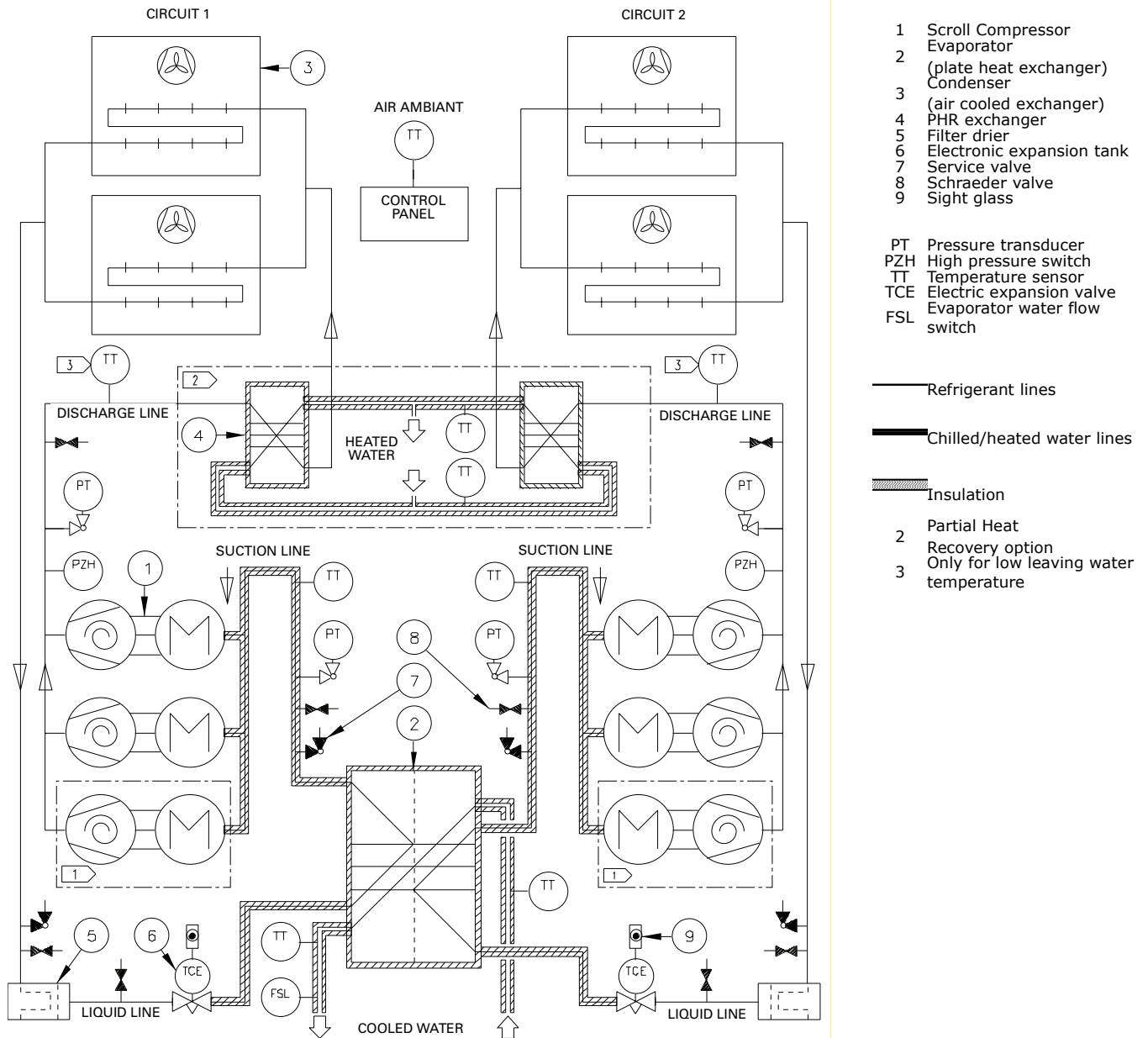
Figure 3. Refrigerant chart cooling only units (CGAM)
