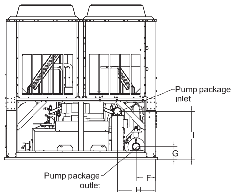
Figure 4. DUPLEX W configuration
