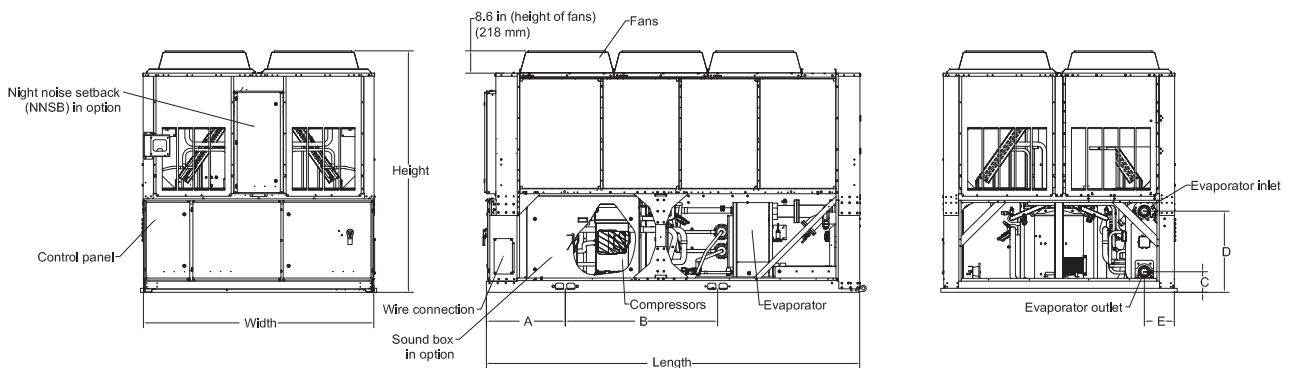
Figure 1. Standard Unit - DUPLEX W configuration
