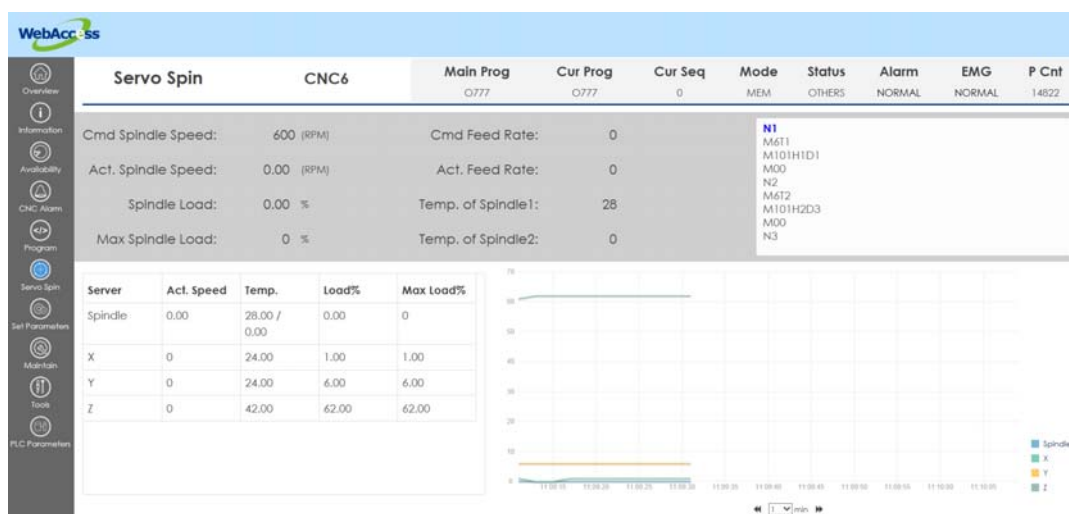
Figure 3.13 Directly access the WebAccess/CNC device information page
