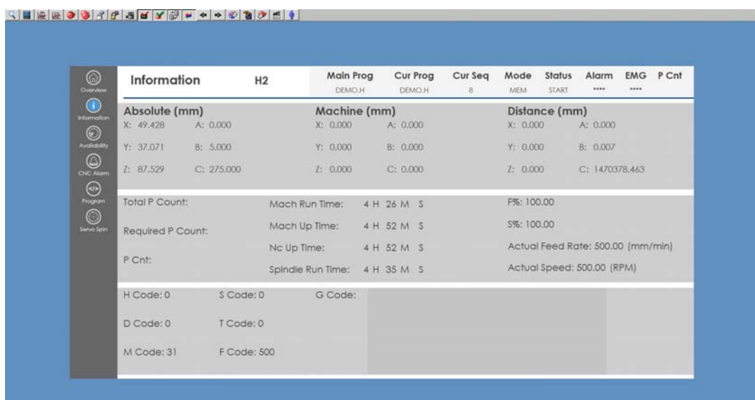
Figure 3.12 Available functions when the setting “menu=224” is applied
