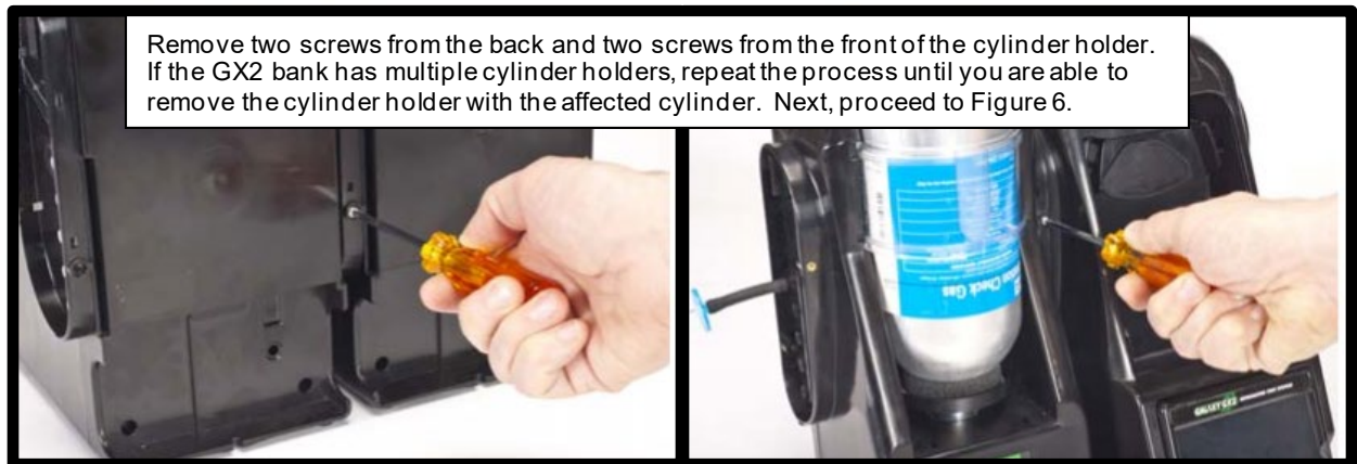
Figure 5 – Removing a Cylinder Holder from a GX2 Bank
