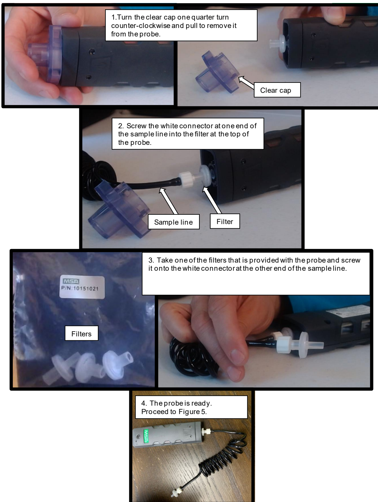
Figure 4 – Preparing the Pump Probe
