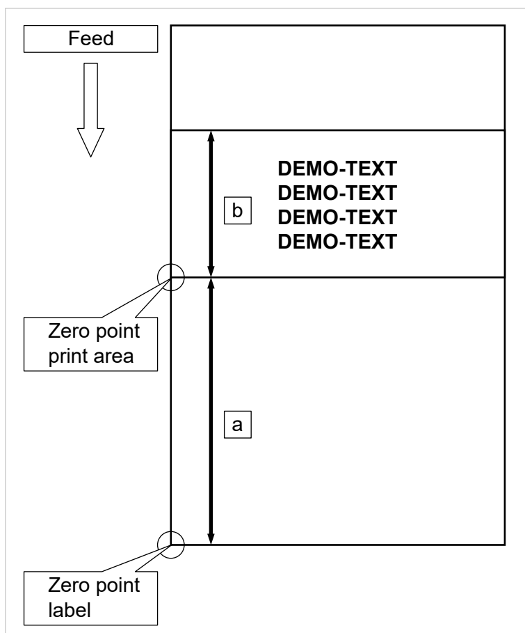
Fig. 10: Offsetting the zero point of the print area with the length „b“ by the distance „a“.
