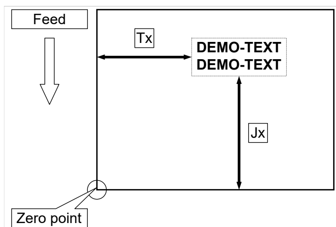
Fig. 15: Vertical (Jx) and horizontal (Tx) print position on the label.
