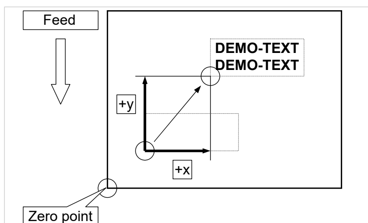
Fig. 11: Shifting a text block in x/y direction.
