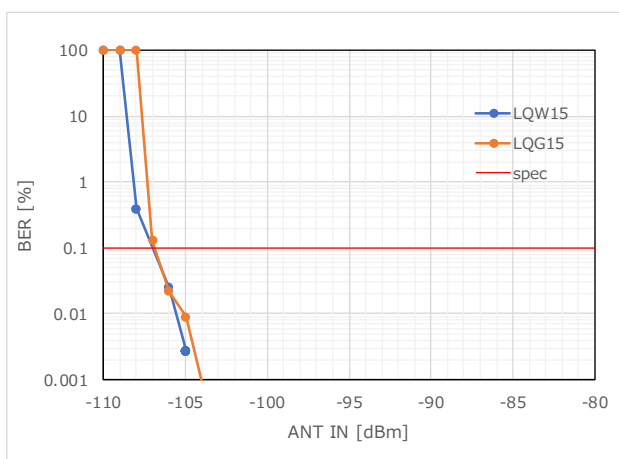
Figure 35 RX Sensitivity_BER (915.0MHz)
