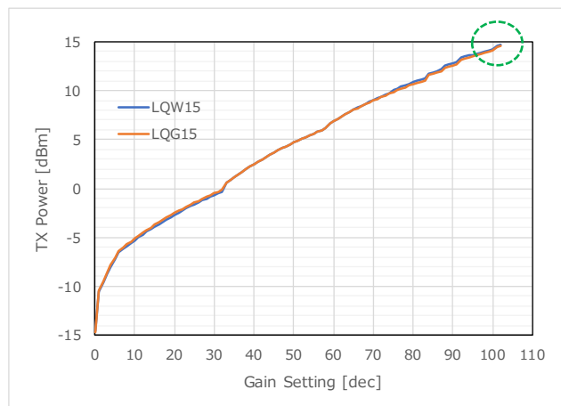
Figure 42 TX Power (875.5MHz)
