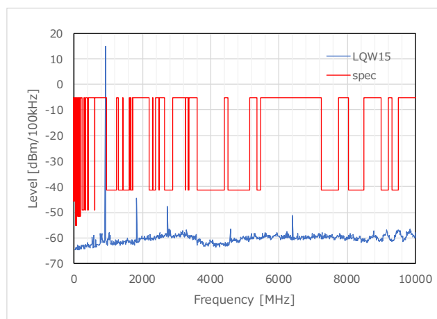
Figure 28 TX Harmonics_LQW15 (915.0MHz)
