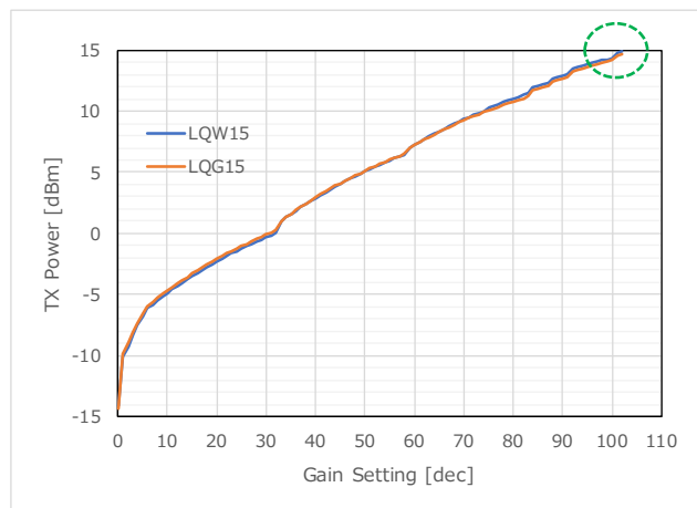
Figure 6 TX Power (875.5MHz)
