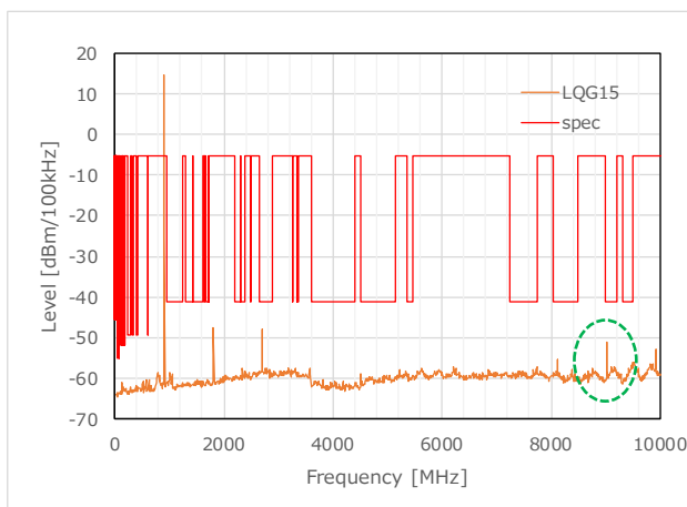
Figure 27 TX Harmonics_LQG15 (902.2MHz)
