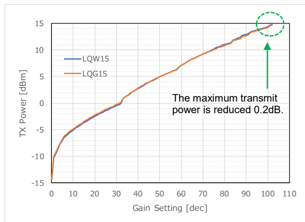
Figure 2 TX Power (863.1MHz)
