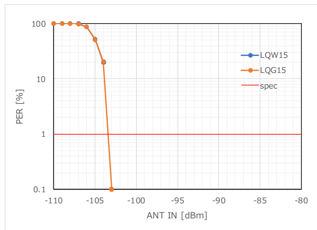
Figure 32 RX Sensitivity_PER (902.2MHz)
