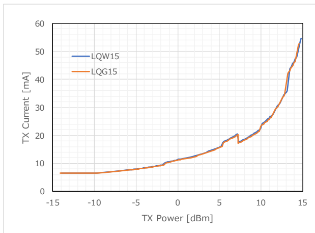
Figure 21 TX Current (902.2MHz)
