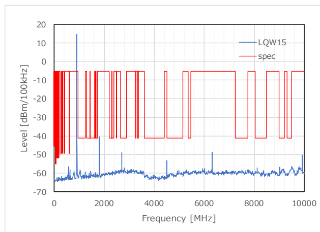
Figure 62 TX Harmonics_LQW15 (902.2MHz)
