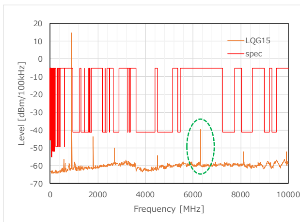
Figure 63 TX Harmonics_LQG15 (902.2MHz)
