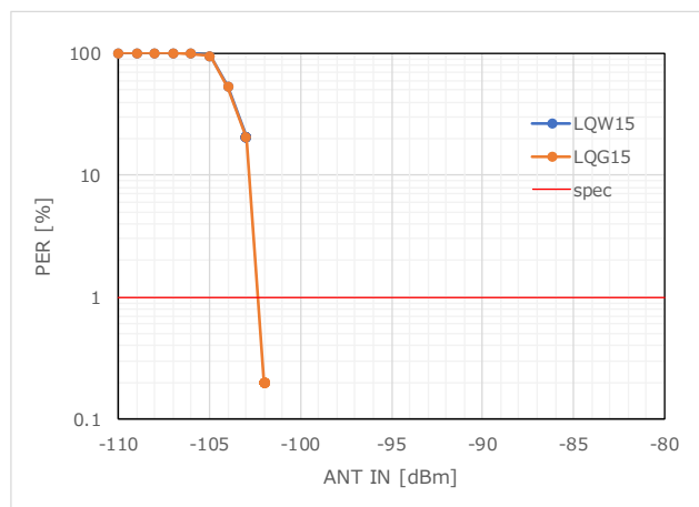
Figure 16 RX Sensitivity_PER (869.3MHz)
