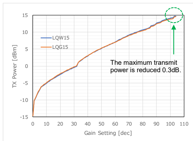
Figure 56 TX Power (902.2MHz)
