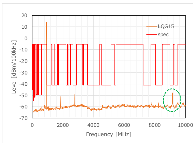
Figure 29 TX Harmonics_LQG15 (915.0MHz)
