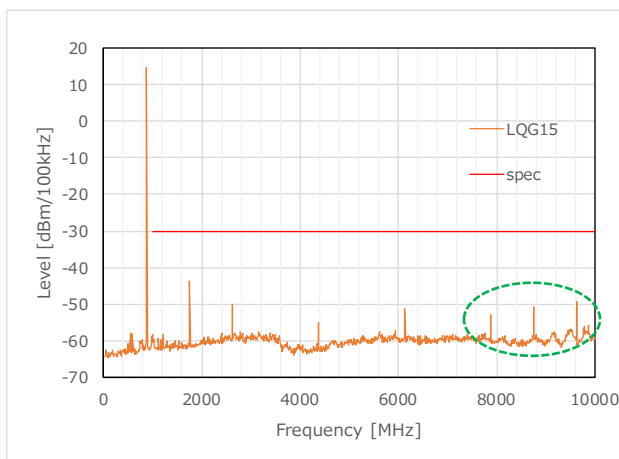
Figure 49 TX Harmonics_LQG15 (875.5MHz)
