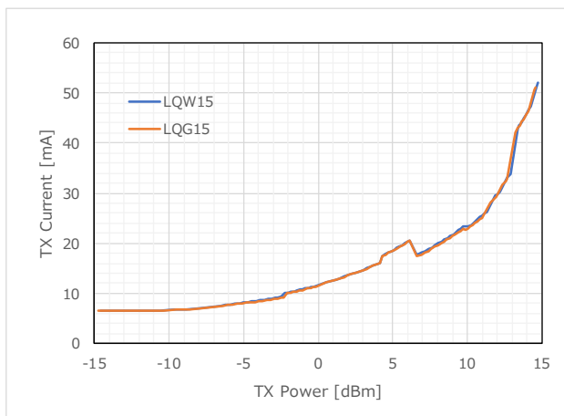
Figure 43 TX Current (875.5MHz)
