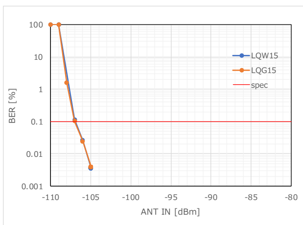
Figure 71 RX Sensitivity_BER (915.0MHz)
