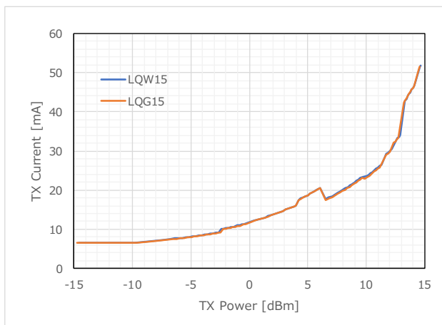
Figure 39 TX Current (863.1MHz)
