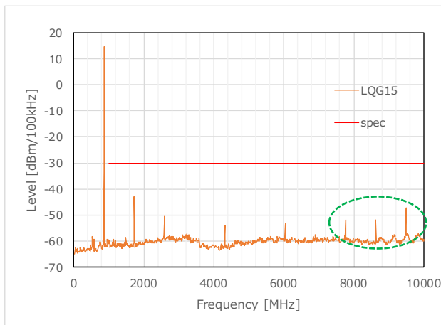
Figure 45 TX Harmonics_LQG15 (863.1MHz)
