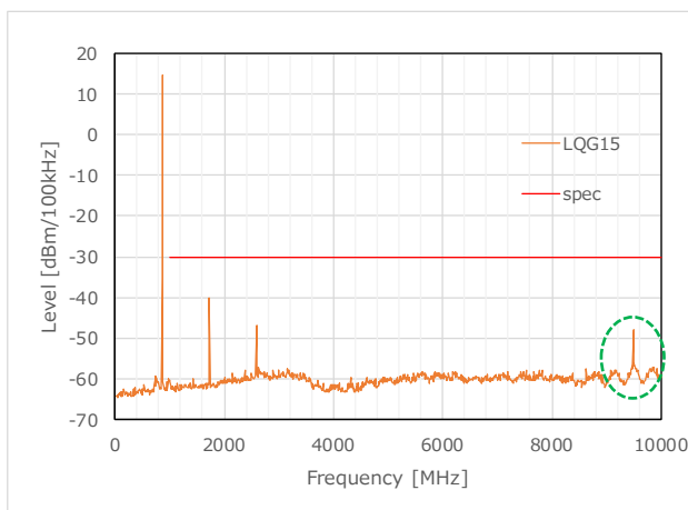
Figure 9 TX Harmonics_LQG15 (863.1MHz)
