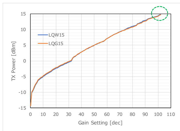
Figure 4 TX Power (869.3MHz)
