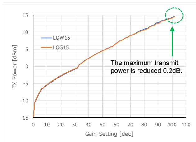
Figure 38 TX Power (863.1MHz)
