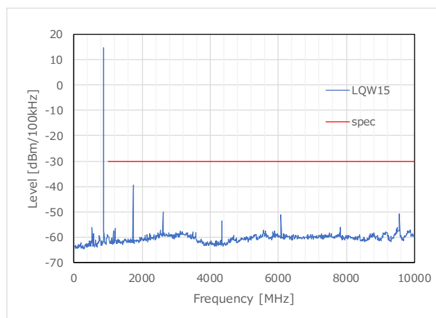
Figure 46 TX Harmonics_LQW15 (869.3MHz)
