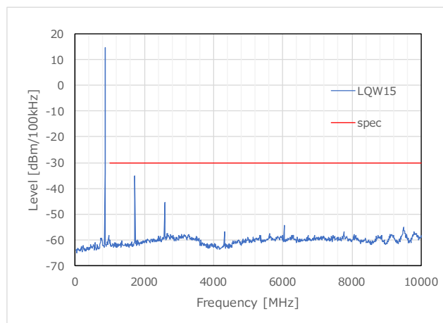
Figure 8 TX Harmonics_LQW15 (863.1MHz)
