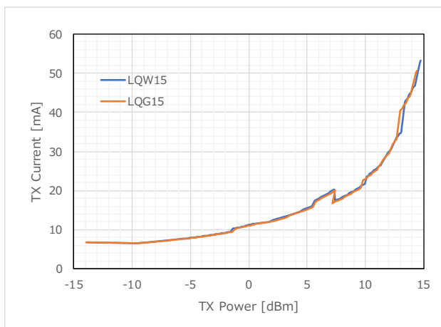
Figure 25 TX Current (927.8MHz)
