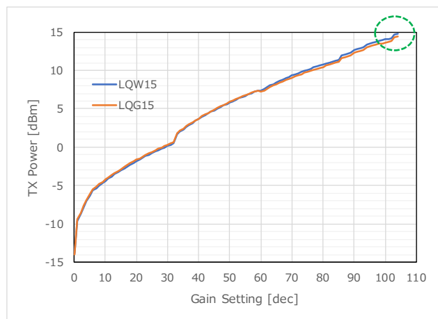
Figure 24 TX Power (927.8MHz)
