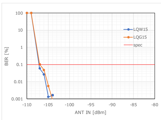
Figure 37 RX Sensitivity_BER (927.8MHz)
