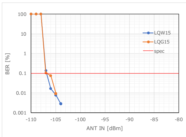
Figure 33 RX Sensitivity_BER (902.2MHz)
