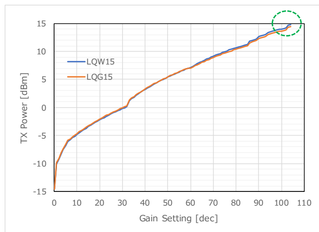
Figure 60 TX Power (927.8MHz)
