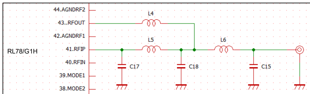
Figure 1 Matching circuit configuration
