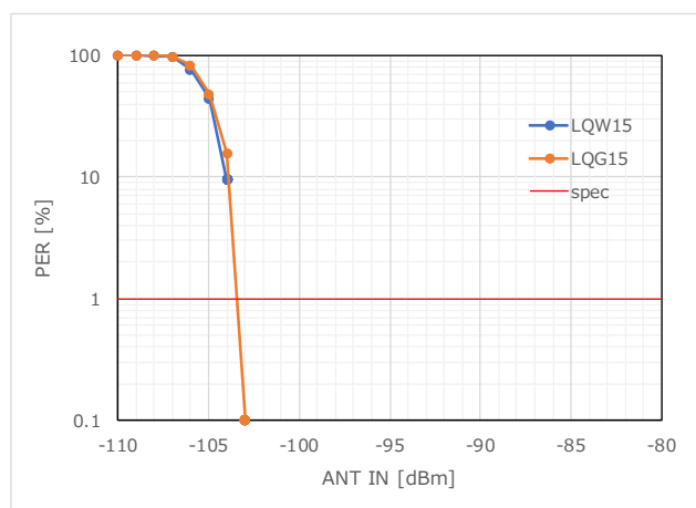
Figure 34 RX Sensitivity_PER (915.0MHz)
