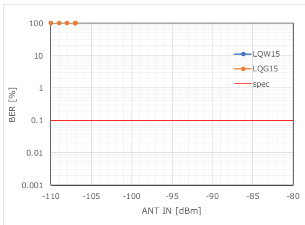
Figure 51 RX Sensitivity_BER (863.1MHz)
