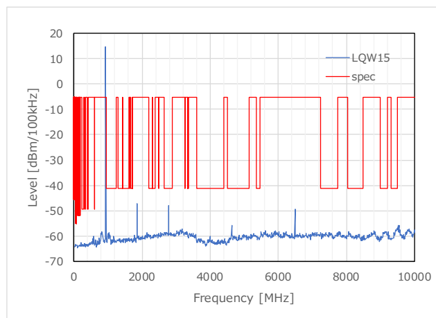
Figure 30 TX Harmonics_LQW15 (927.8MHz)
