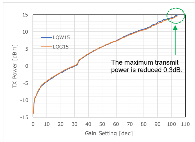
Figure 20 TX Power (902.2MHz)
