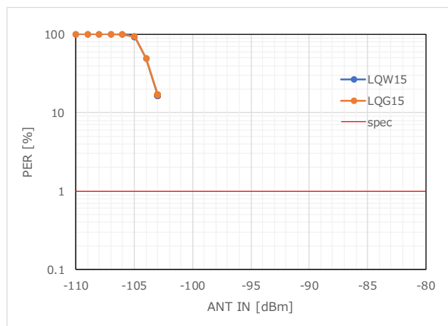
Figure 52 RX Sensitivity_PER (869.3MHz)
