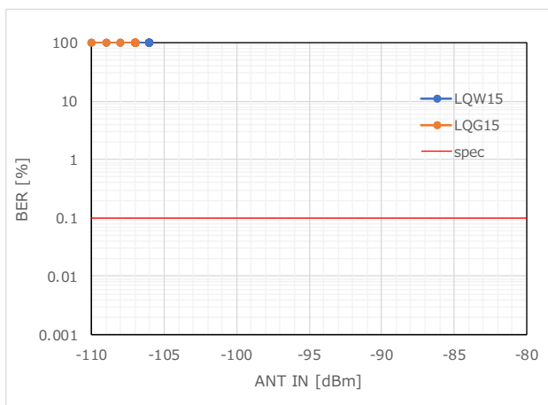
Figure 17 RX Sensitivity_BER (869.3MHz)
