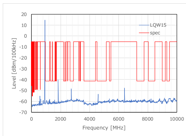
Figure 64 TX Harmonics_LQW15 (915.0MHz)
