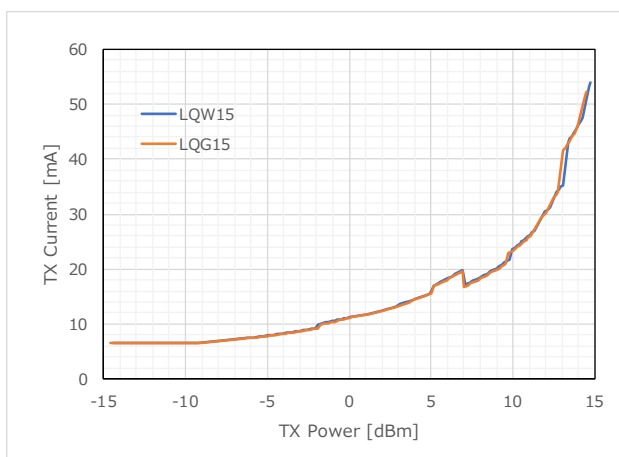
Figure 59 TX Current (915.0MHz)
