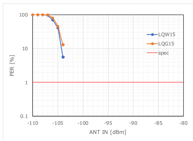
Figure 36 RX Sensitivity_PER (927.8MHz)
