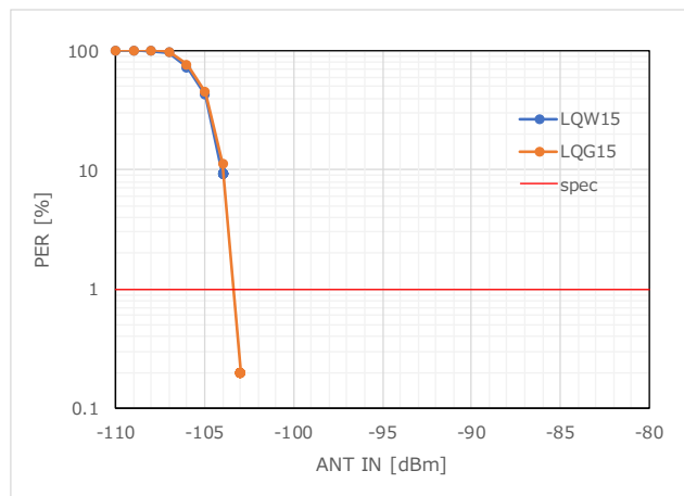
Figure 68 RX Sensitivity_PER (902.2MHz)
