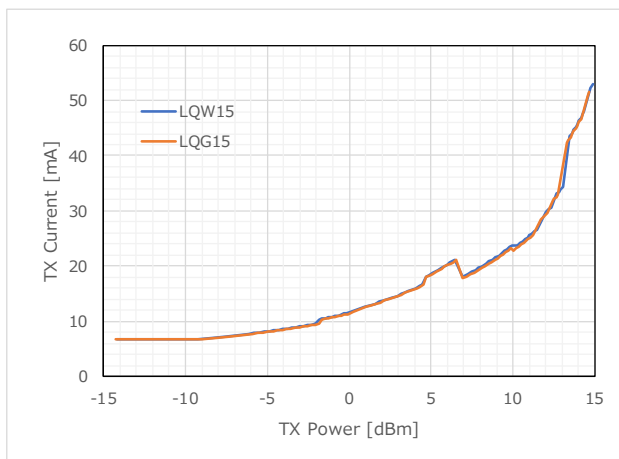
Figure 7 TX Current (875.5MHz)
