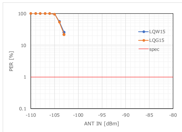
Figure 50 RX Sensitivity_PER (863.1MHz)
