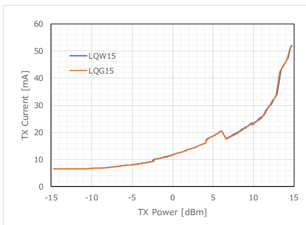
Figure 41 TX Current (869.3MHz)
