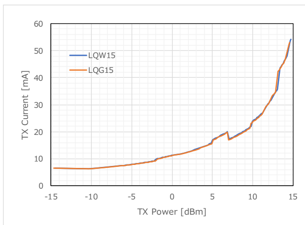
Figure 57 TX Current (902.2MHz)
