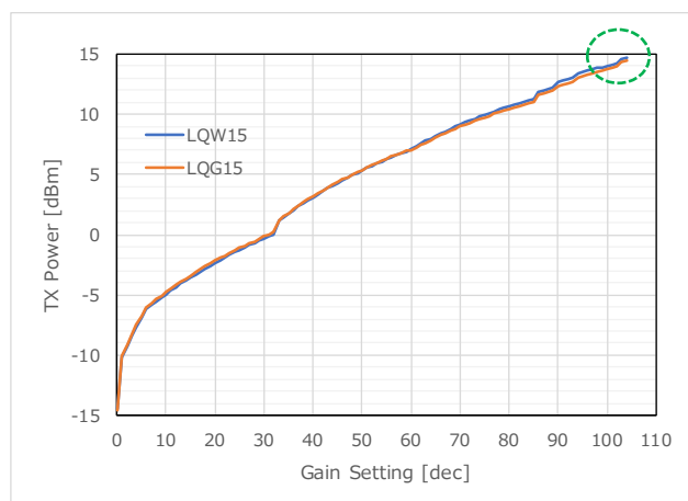
Figure 58 TX Power (915.0MHz)
