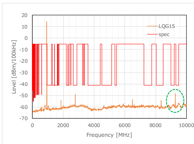
Figure 31 TX Harmonics_LQG15 (927.8MHz)
