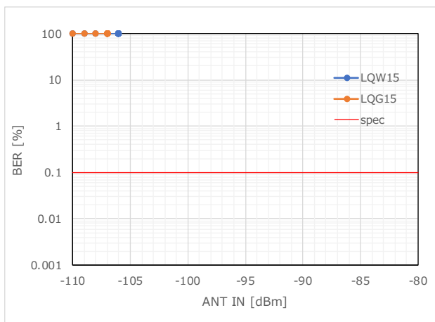
Figure 19 RX Sensitivity_BER (875.5MHz)
