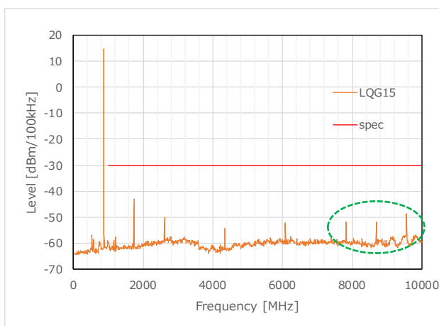
Figure 47 TX Harmonics_LQG15 (869.3MHz)
