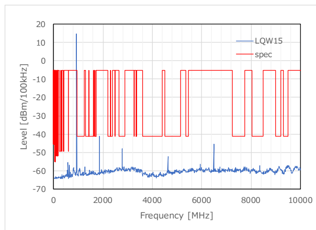
Figure 66 TX Harmonics_LQW15 (927.8MHz)
