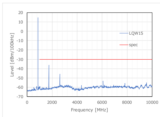
Figure 10 TX Harmonics_LQW15 (869.3MHz)
