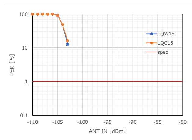
Figure 18 RX Sensitivity_PER (875.5MHz)
