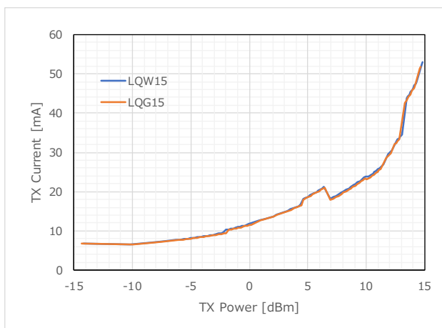
Figure 5 TX Current (869.3MHz)
