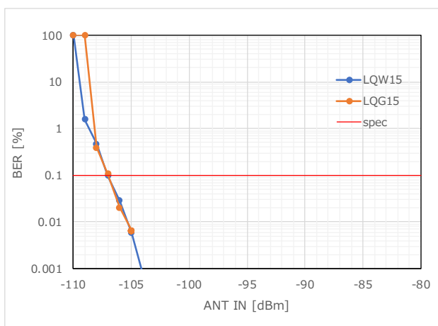
Figure 73 RX Sensitivity_BER (927.8MHz)
