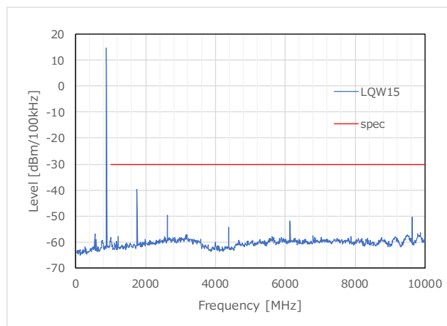
Figure 48 TX Harmonics_LQW15 (875.5MHz)
