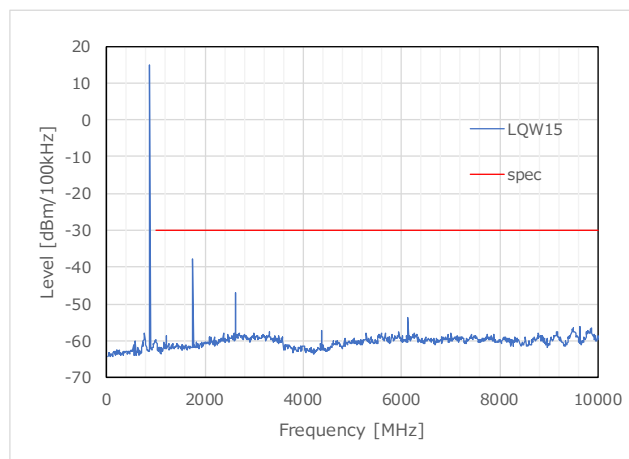
Figure 12 TX Harmonics_LQW15 (875.5MHz)
