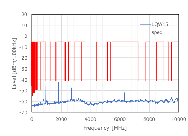
Figure 26 TX Harmonics_LQW15 (902.2MHz)
