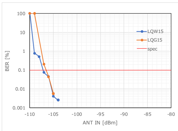
Figure 69 RX Sensitivity_BER (902.2MHz)
