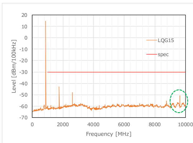
Figure 13 TX Harmonics_LQG15 (875.5MHz)
