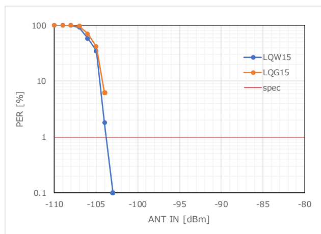
Figure 72 RX Sensitivity_PER (927.8MHz)
