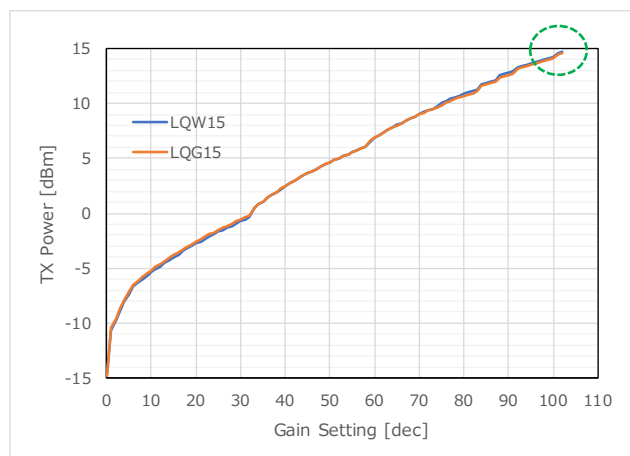
Figure 40 TX Power (869.3MHz)
