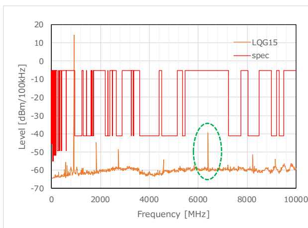
Figure 65 TX Harmonics_LQG15 (915.0MHz)
