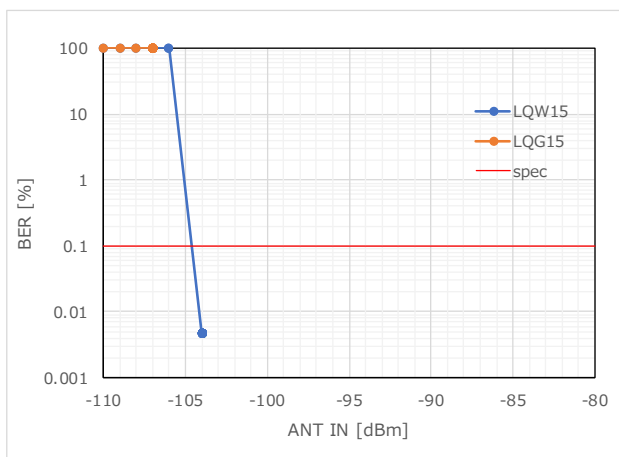
Figure 53 RX Sensitivity_BER (869.3MHz)
