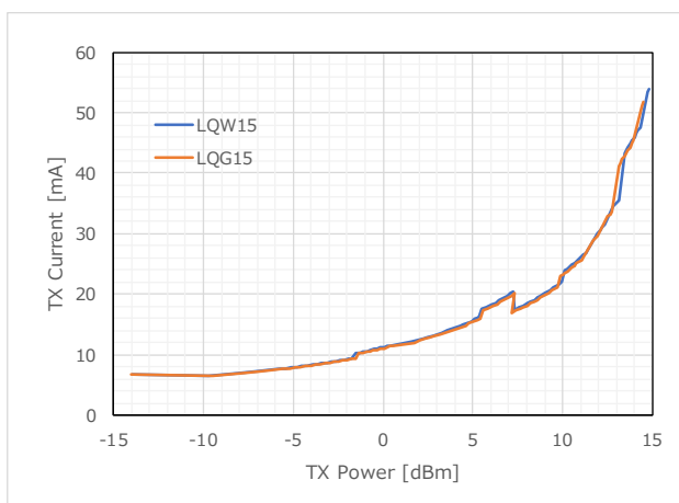
Figure 23 TX Current (915.0MHz)
