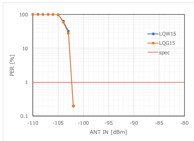
Figure 14 RX Sensitivity_PER (863.1MHz)
