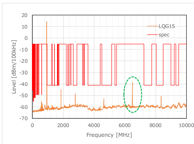
Figure 67 TX Harmonics_LQG15 (927.8MHz)
