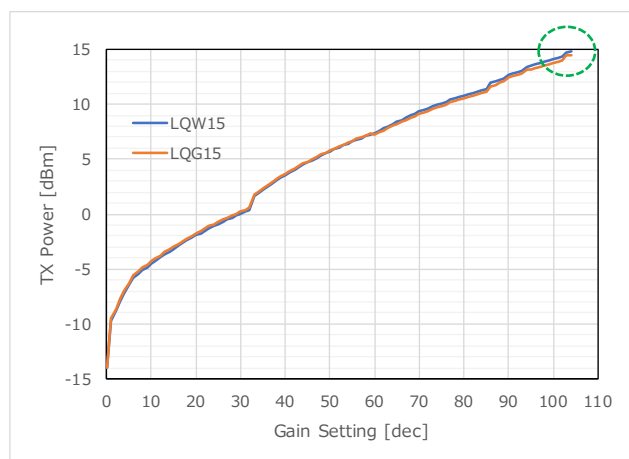
Figure 22 TX Power (915.0MHz)
