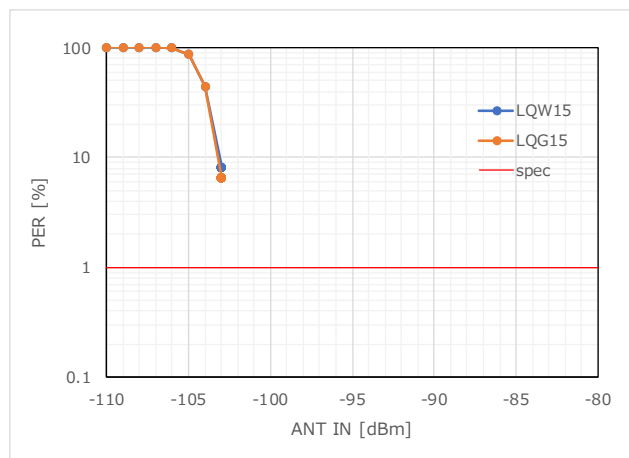
Figure 54 RX Sensitivity_PER (875.5MHz)
