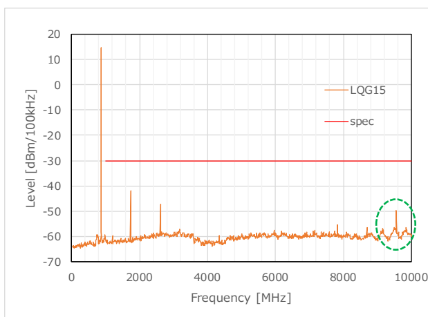
Figure 11 TX Harmonics_LQG15 (869.3MHz)
