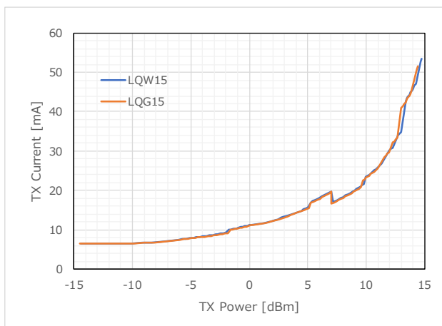
Figure 61 TX Current (927.8MHz)
