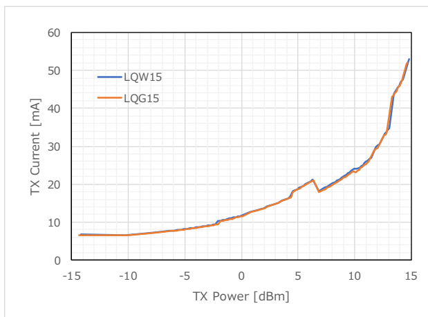
Figure 3 TX Current (863.1MHz)
