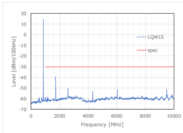
Figure 44 TX Harmonics_LQW15 (863.1MHz)
