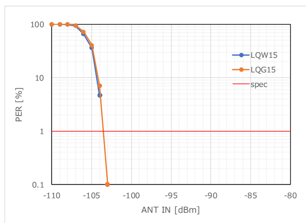
Figure 70 RX Sensitivity_PER (915.0MHz)
