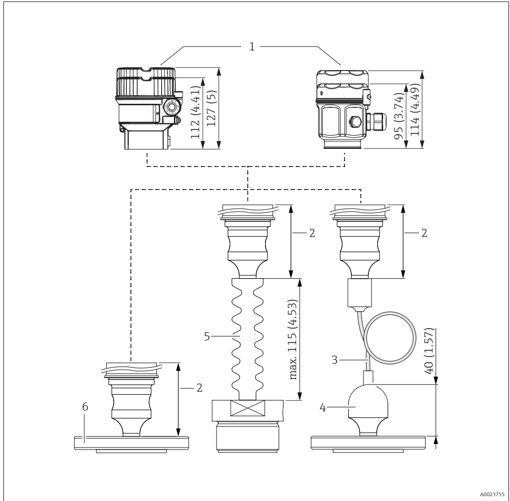
PMP55 basic device with diaphragm seal
