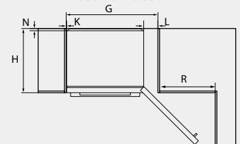
Plan View Flush with refrigerator door - 90° door rotation
