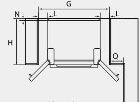
Plan View Flush with refrigerator door - 90° door rotation
