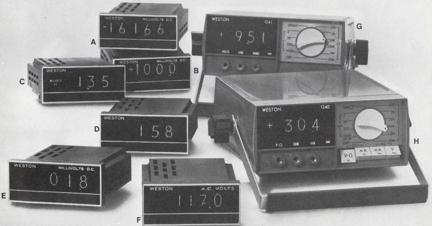
A. 4 1/2-digit bi-polar Model 1294 B. 3 1/2-digit bi-polar Model 1292 C. 2 1/2-digit Model 1260 D. Event Counter Model 1266 E. 3-digit Model 1261 F. AC Line Monitor Model 1262 G. Digital VOM Model 1241 H. Digital Multimeter Model 1240
