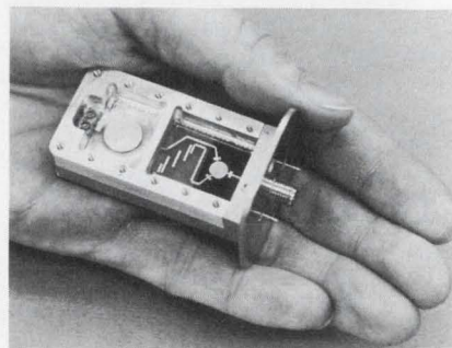
Doppler radar with Gunn diode produces 50 mW at 10.525 GHz.
