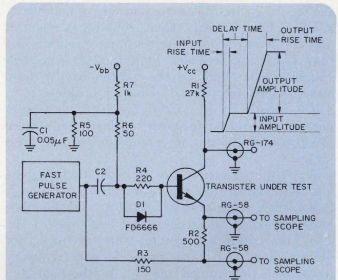
Measurement of the characteristics of transistors operating in the avalanche mode is simplified by displaying both amplitude and timing parameters simultaneously on a single oscilloscope beam.
