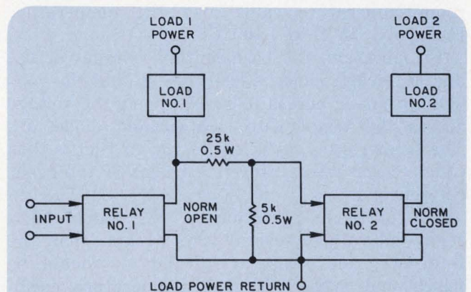
With no input, relay No. 2 is kept energized by the trickle current through load No. 1. This keeps load No. 2 normally on.
