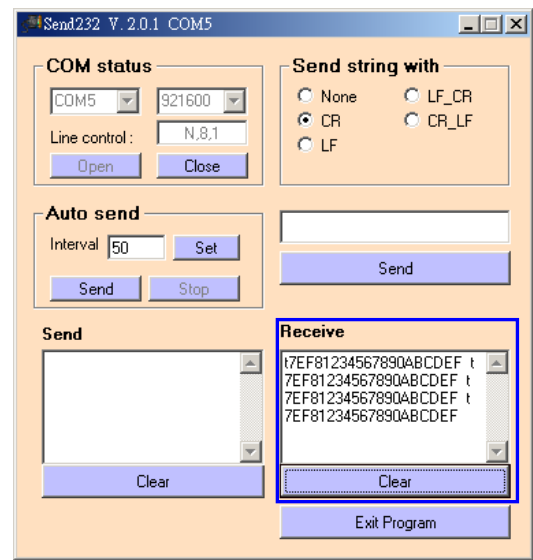
Figure 6-4: Send Messages from RS-232 to CAN
