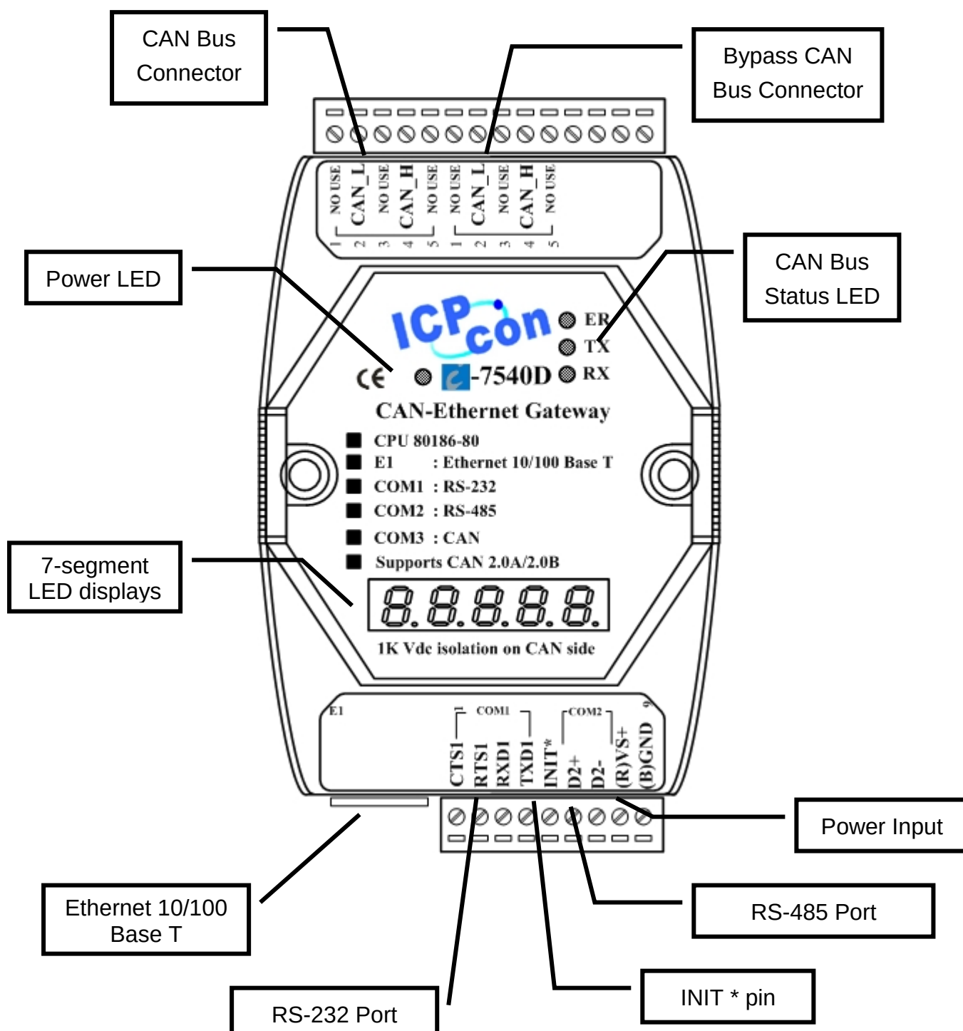
Figure 2-2: Pin assignment on the I-7540D
