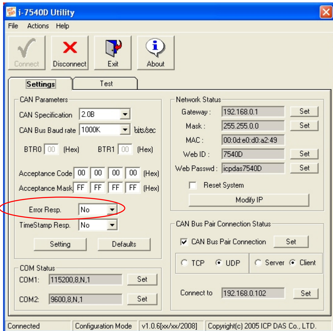
Figure 3-16: Error Response
