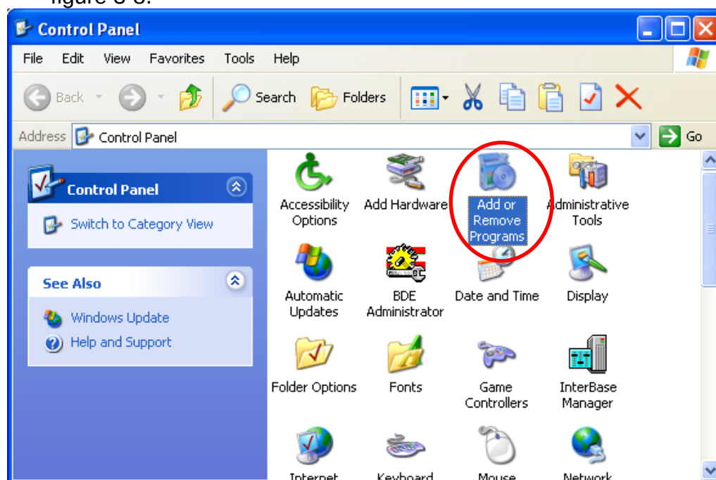
Figure 3-8: “Add/Remove Programs”
