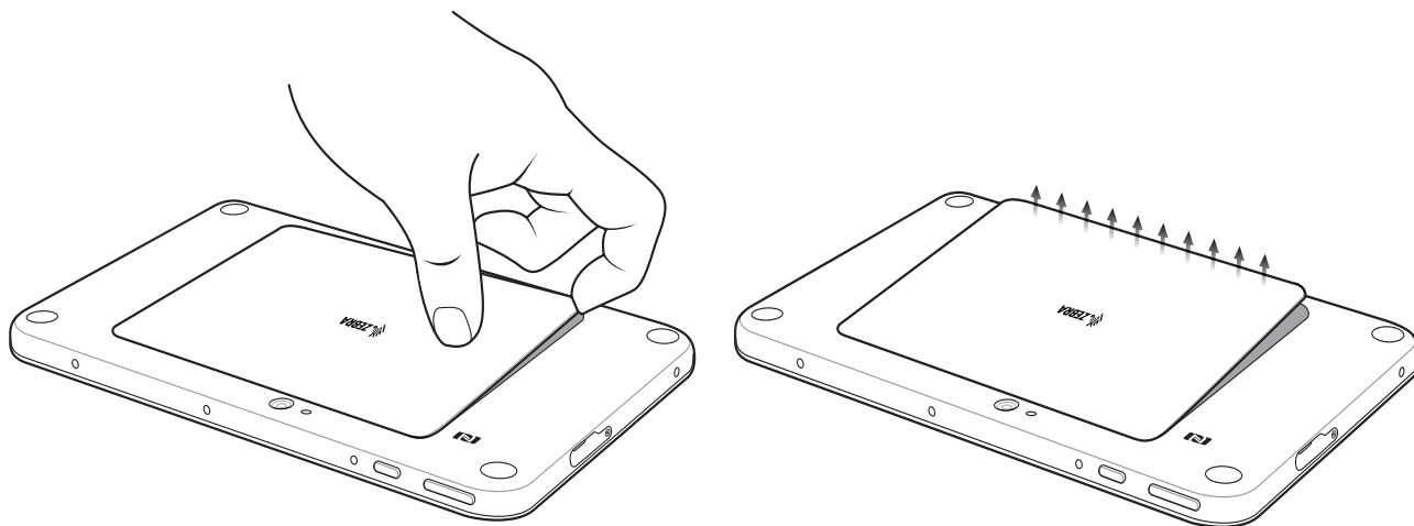
Figure 4 Lifting the Battery Cover
