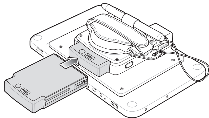
Figure 76 Install Power Pack
