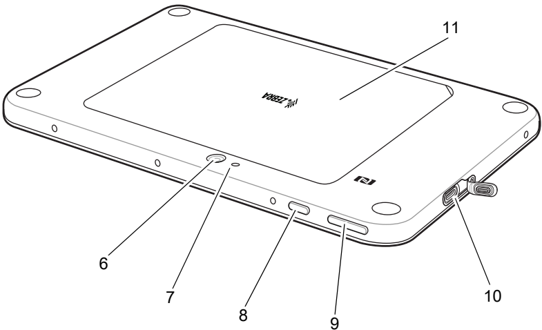
Figure 2 Back View
