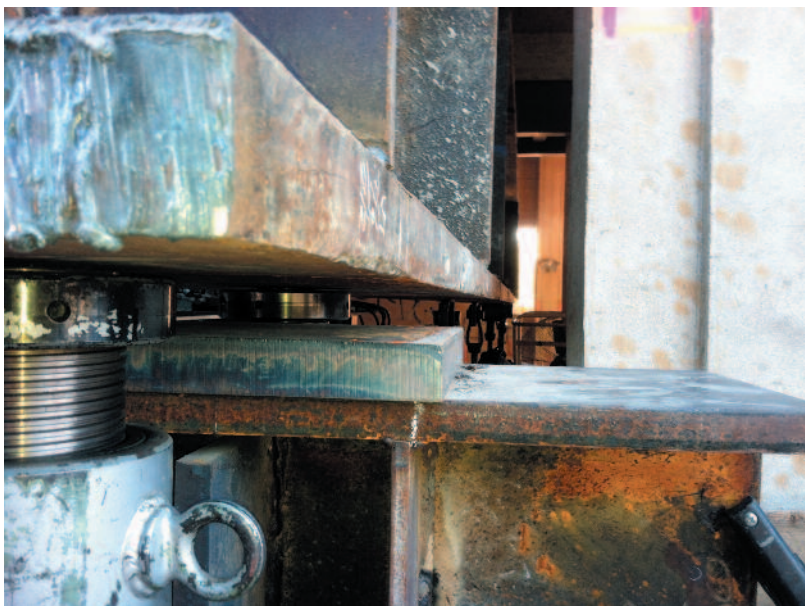
Jacking the W36 needle girders using two hydraulic jacks to lift each end of the beam. Under the weight of the building, the middle of the beam did not move.
