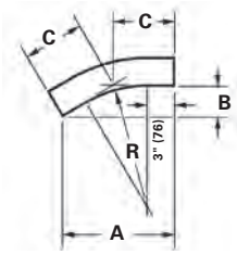
30° Vertical Outside
