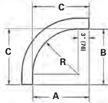
90° Vertical Outside
