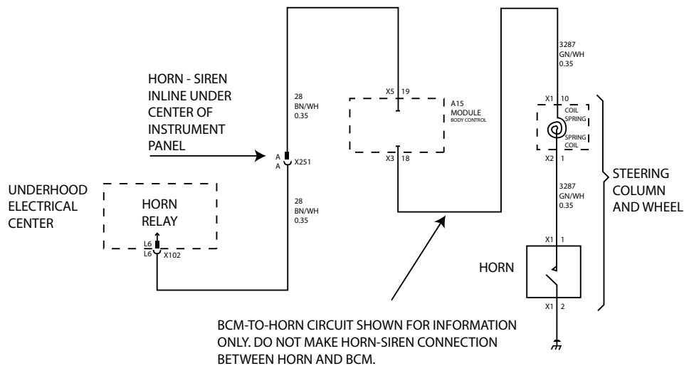
WIRING PROVISION FOR OPTION 6J4, HORN - SIREN CIRCUIT
