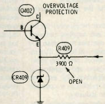
6 Chassis—RCA CTC58 PHOTOFACT—1365-1 (1428-2)
