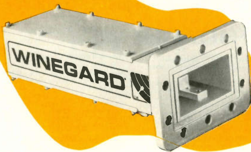
Figure 1. The LNA is a pre-amplifier that must be located directly at the antenna; otherwise, the received signal, which is extremely small, would be so attenuated and swamped by noise by the time it reached the TV set that it would be unusable. It is called a low-noise amplifier because it must contribute very little noise to the small-amplitude received signal that it amplifies, or it would contribute enough noise to make the signal unwatchable.
