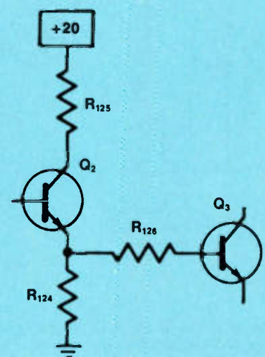
Figure 1. A manufacturer's schematic or Sams Photofact schematic contains a lot of information about a consumer electronics product. The purpose and operation of a particular segment of the circuitry is frequently obscured, however, because the circuit contains more information than you need, or is drawn in an unfamiliar orientation. You can enhance your understanding of a circuit by drawing a simplified schematic diagram in an orientation that you're comfortable with.
