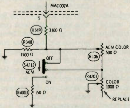
1 Chassis—RCA CTC71 PHOTOFACT—1380-2 (1435-3)
