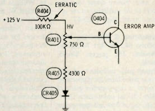
4 Chassis—RCA CTC76 PHOTOFACT—1468-2 (1519-2)
