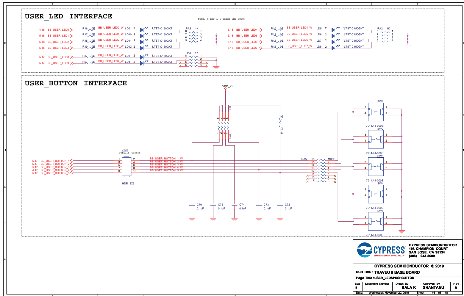
Figure C-14. USER_LED &amp; PUSHBUTTON
