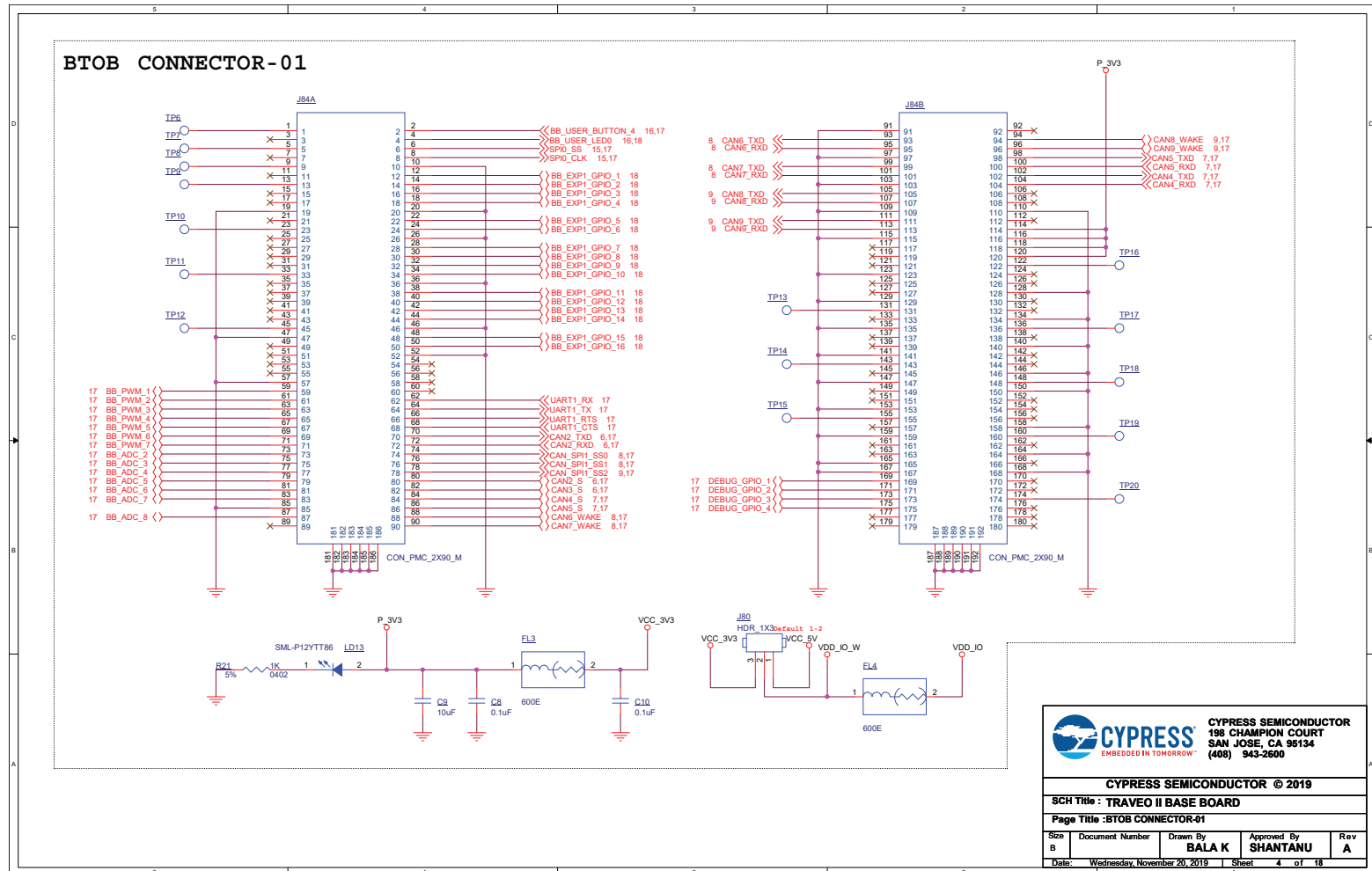
Figure C-2. BTOB Connector-01
