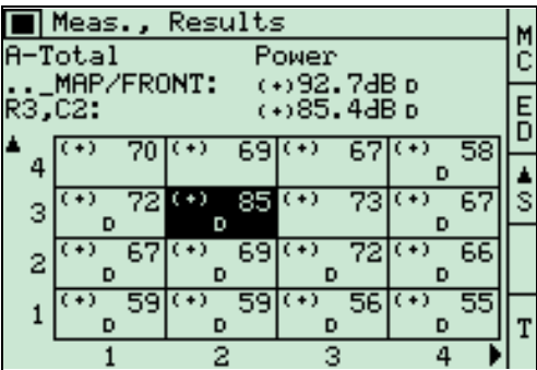
Fig. 11 Sound power measurement results for a 4 × 4 grid
