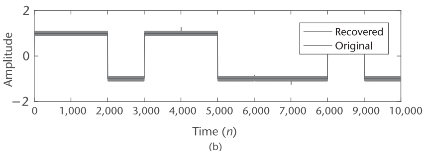
Figure 4.11 Example of quadrature amplitude modulation waveform using an in-phase/quadrature receiver. (a) In-phase signal component, and (b) quadrature signal component.
