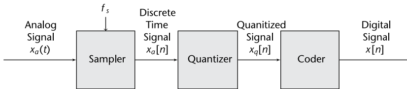
Figure 2.5 Basic parts of an analog-to-digital converter (ADC) [1]. Sampling takes place in the sampler block. x_a(t) = analog continuous time signal; f_s is the digital sample rate; x_a[n] is the discrete time continuous analog signal; x_q[n] is the discrete time, discrete digital signal, which may come out as grey code; and x[n] is the output of the coder in 2s complement form [7].
