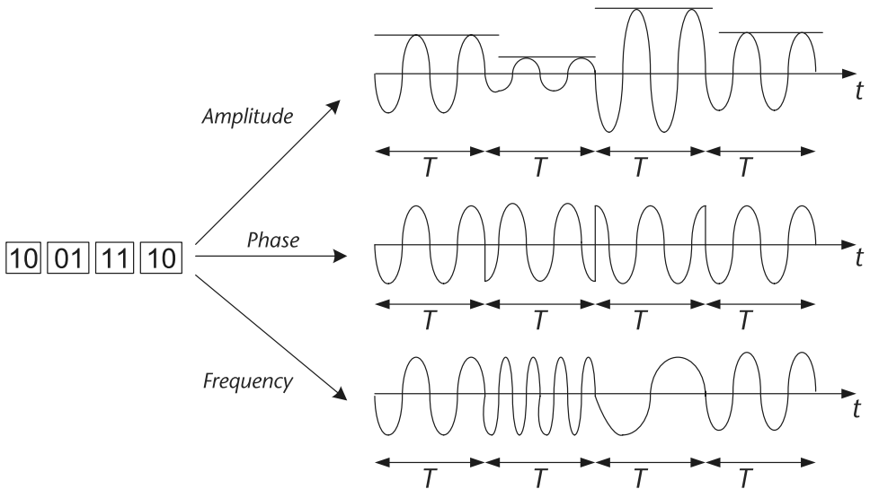
Figure 4.1 Possible mappings of binary information to EM wave properties.
