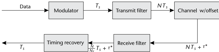
Figure 6.16 Relative rates of transmit and receive chains with respect to the sample rate at different stages. Here \tau^* represents a timing shift not an increase in the data rate. This is a slight abuse of notation.
