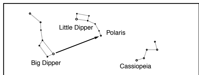
Figure 22: Locating Polaris
