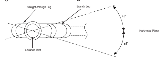
Figure 21: Horizontal Configuration.
