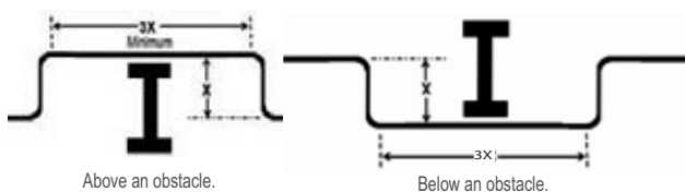
Figure 28: Installing Piping Above and Below an Obstacle.
