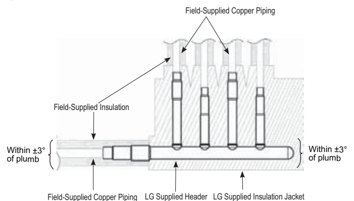
Figure 25: Header Insulation and Pipe Detail.
