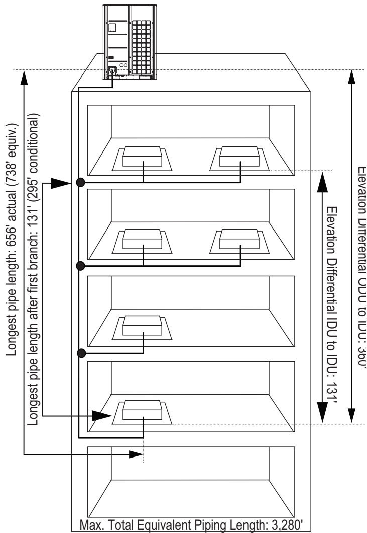
Figure 16: Typical VRF Heat Pump System Building Layout Listing the Piping Limitations.
