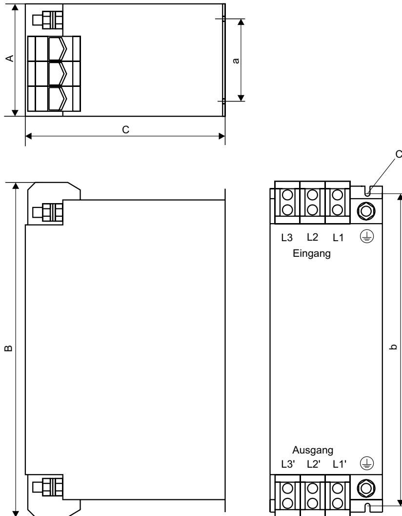
Figure 30: Dimension drawing for NF line filter Any mounting position
