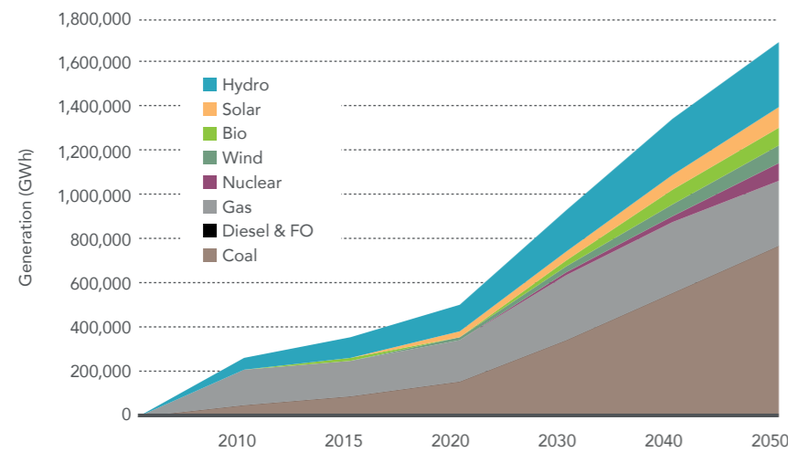
7.5. Generation over time and mix of generation sources between the business-as-usual (BAU; top) and sustainable energy scenario (SES; below). Note that energy efficiency is a high priority for the SES and thus overall demand for the SES is about 30% lower than for the BAU. This will require relatively small improvements in efficiency each year until the region attains levels of efficiency found in other developed Asian countries (from WWF 2016).
