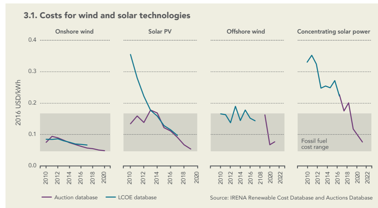
3.1. The Levelized Cost of Energy (LCOE) and auction prices (winning bids) for projects already commissioned or contracted to be commissioned, between 2010 and 2022. For the key commercially available solar and wind technologies, average
