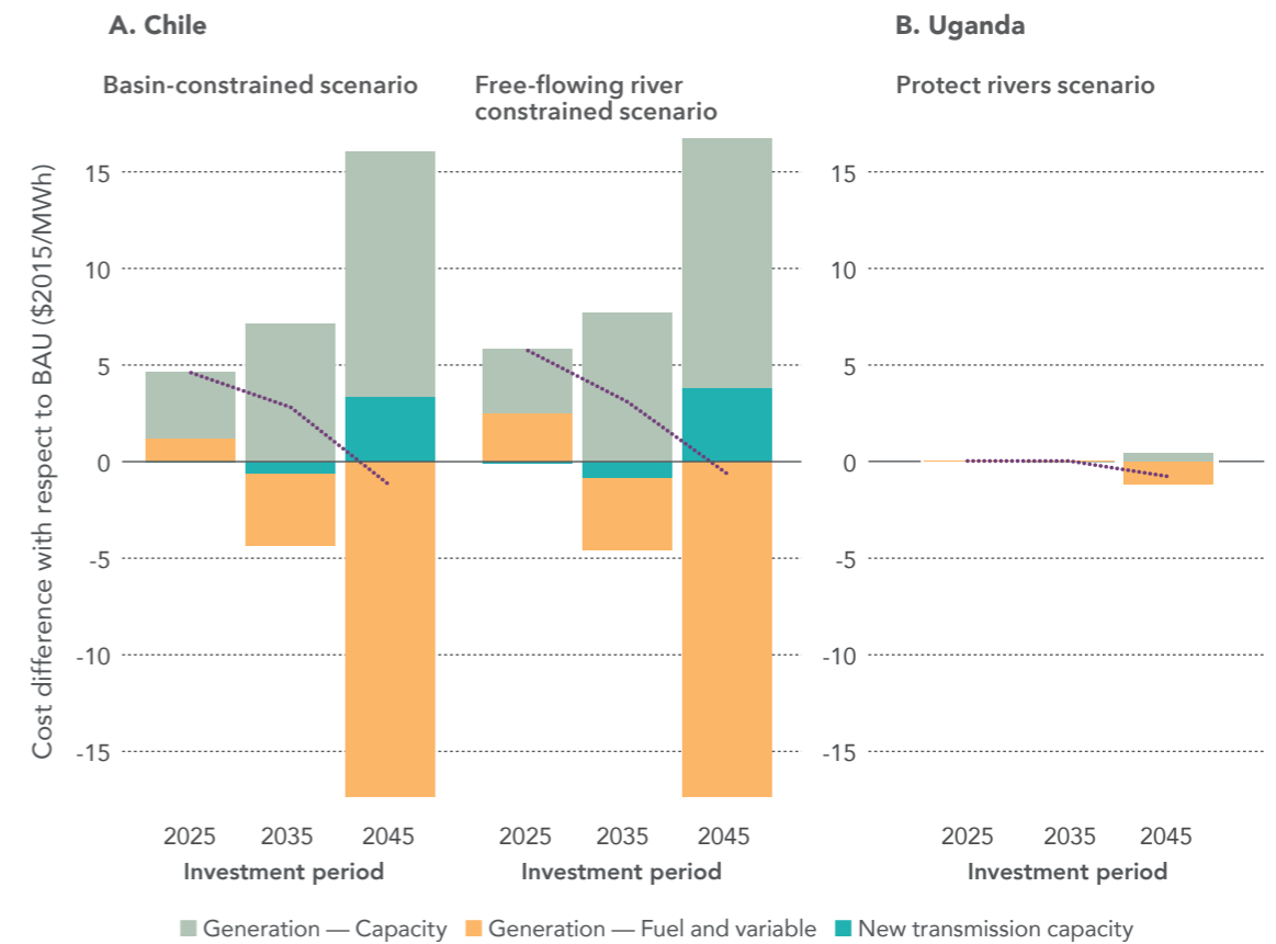
A. Cost difference between low-carbon, low-impact scenarios and the reference scenario, by period and cost type, for Chile.
