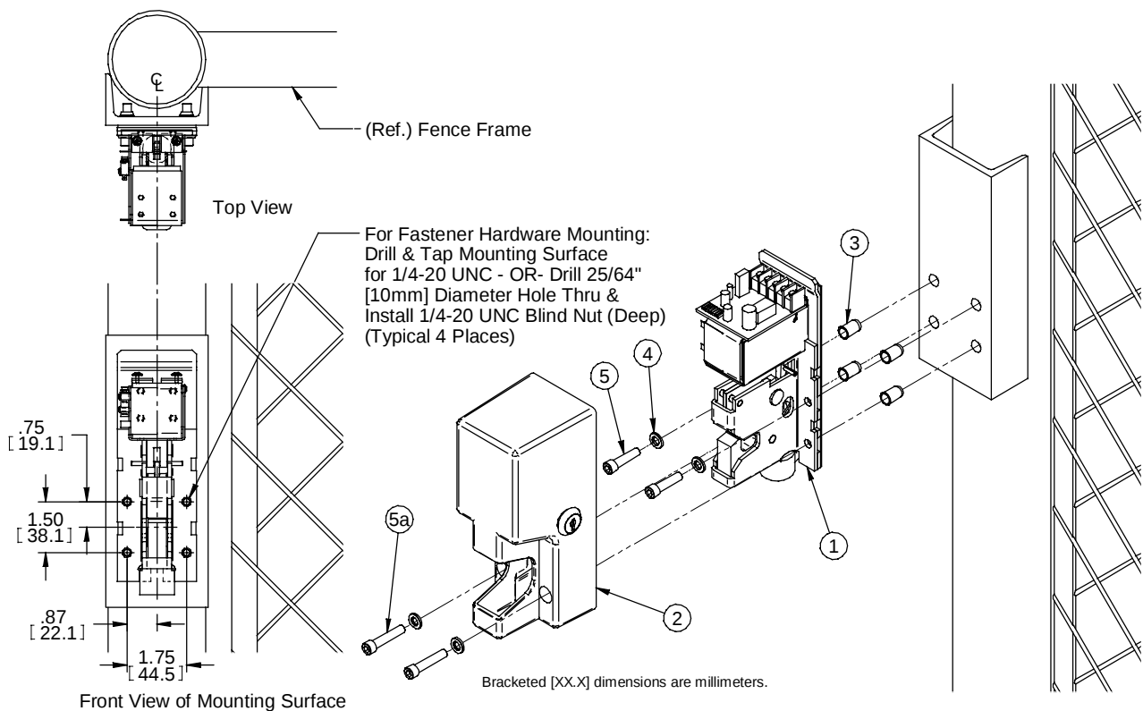
Figure 2 – Lock Installation
