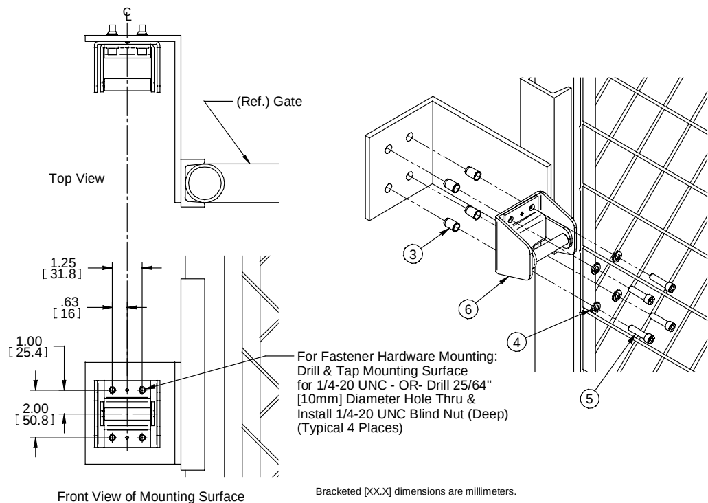
Figure 3 – Strike Installation
