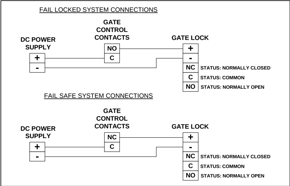
Figure 10 – Wiring Diagram
