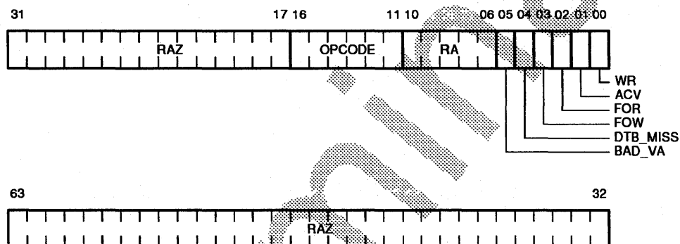
Figure 5-32 Dstream Memory Management Fault Status (MM_STAT) Register
