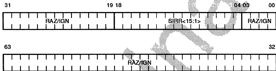
Figure 5-21 Software Interrupt Request Register (SIRR)
