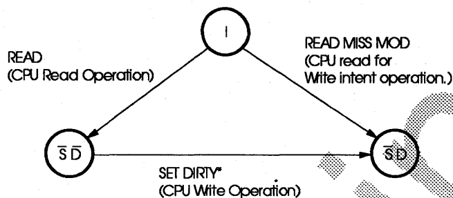
Figure 4-13 Flush-Based Protocol 21164 States
