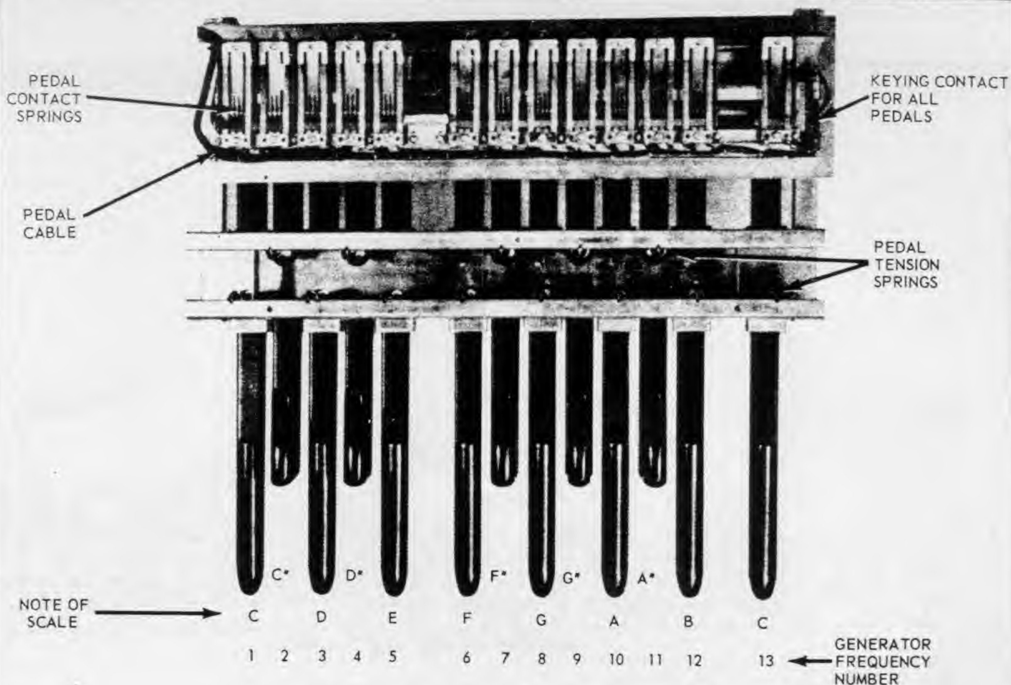
FIGURE 21. PEDAL KEY BOARD MODEL M-100
