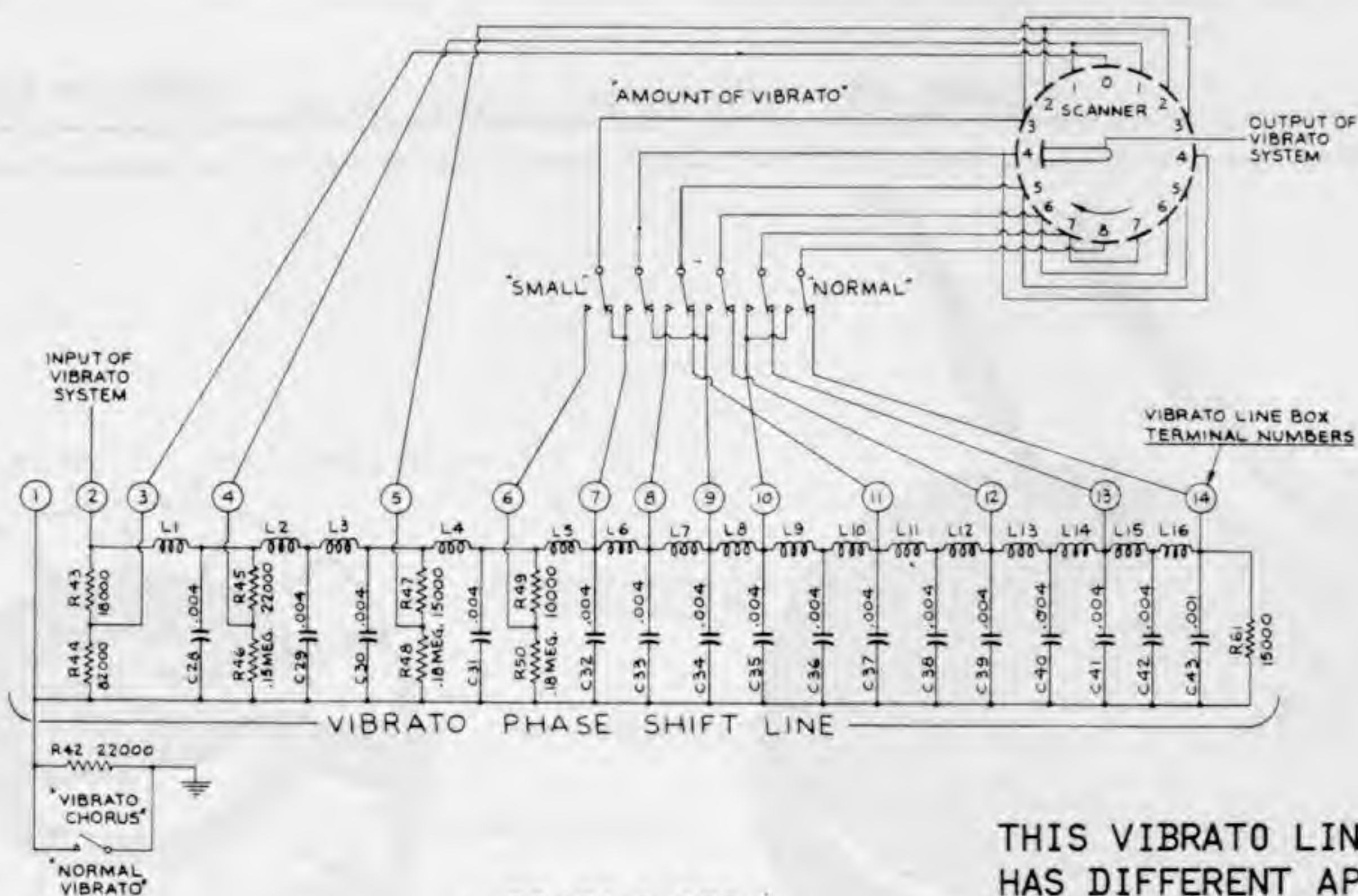
VIBRATO SYSTEM MODEL M-2 CONSOLES SERIAL NUMBER 25254 AND ABOVE
