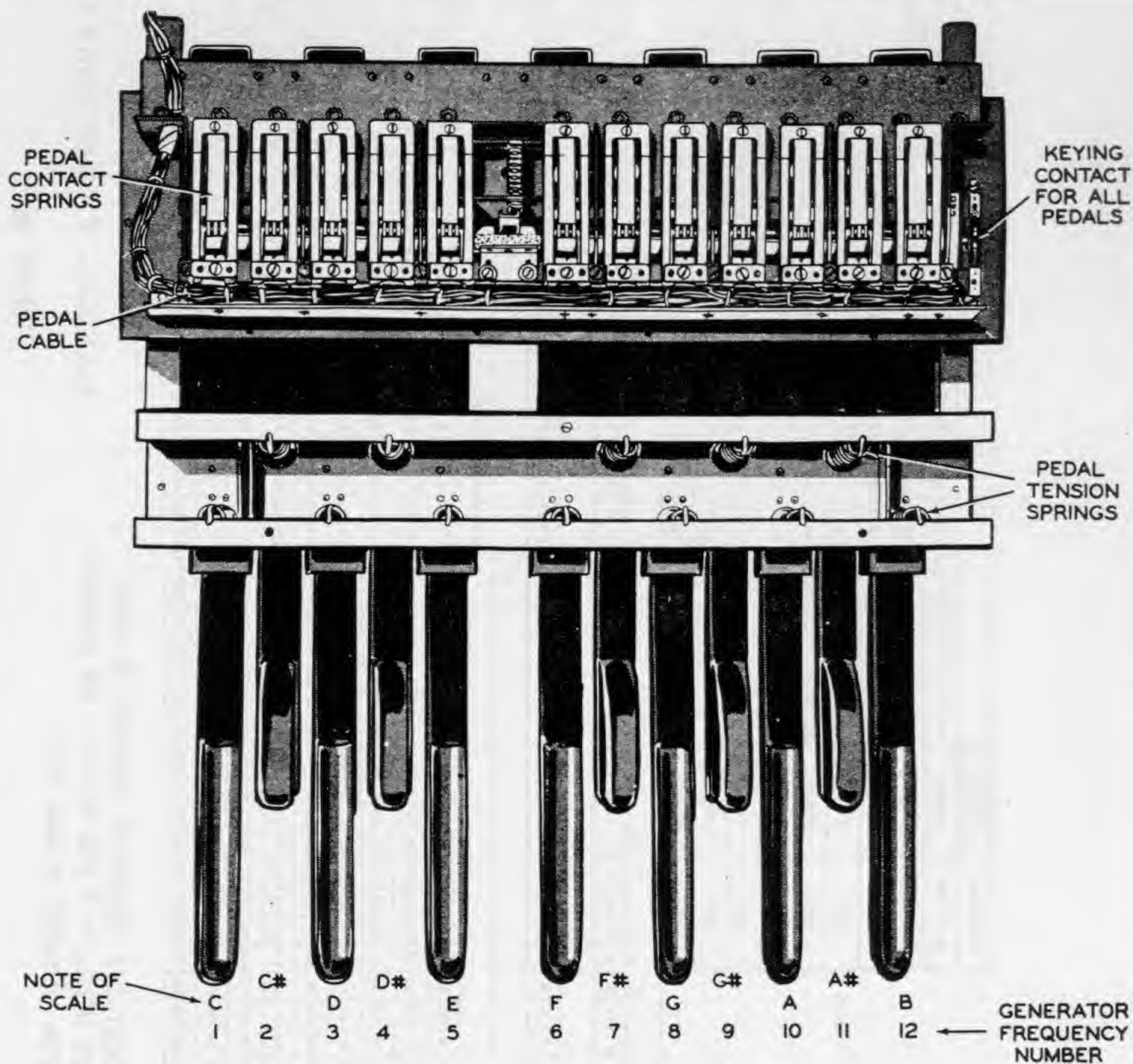
PEDAL KEYBOARD — MODEL M, M-2, AND M-3
