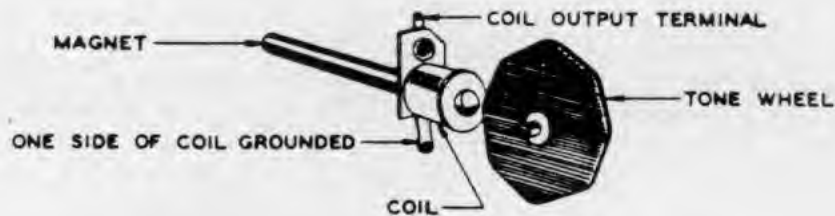
FIGURE 12 - TYPICAL TONE GENERATOR
