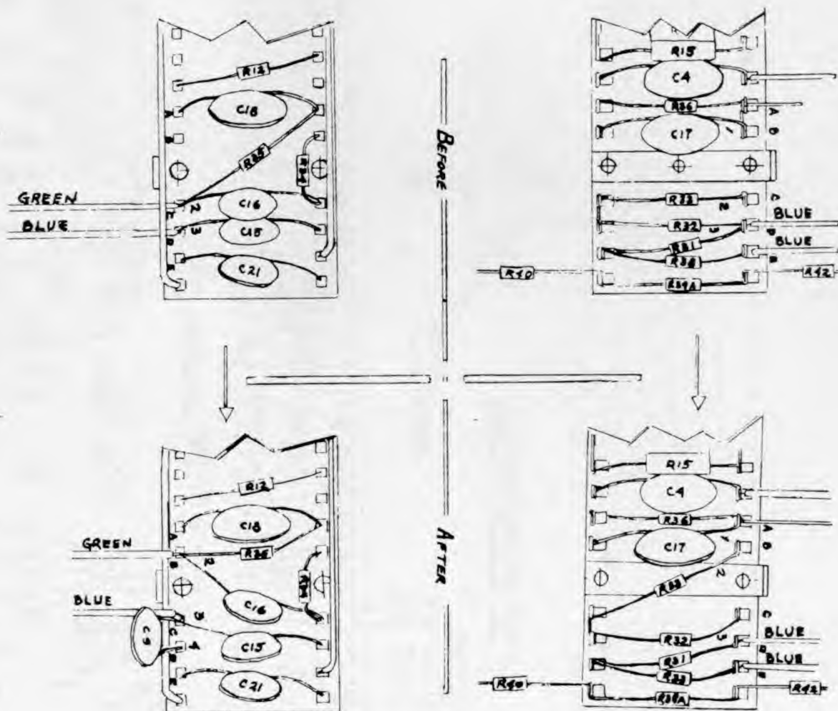
PICTORIAL M-3 AMP (PARTIAL)
