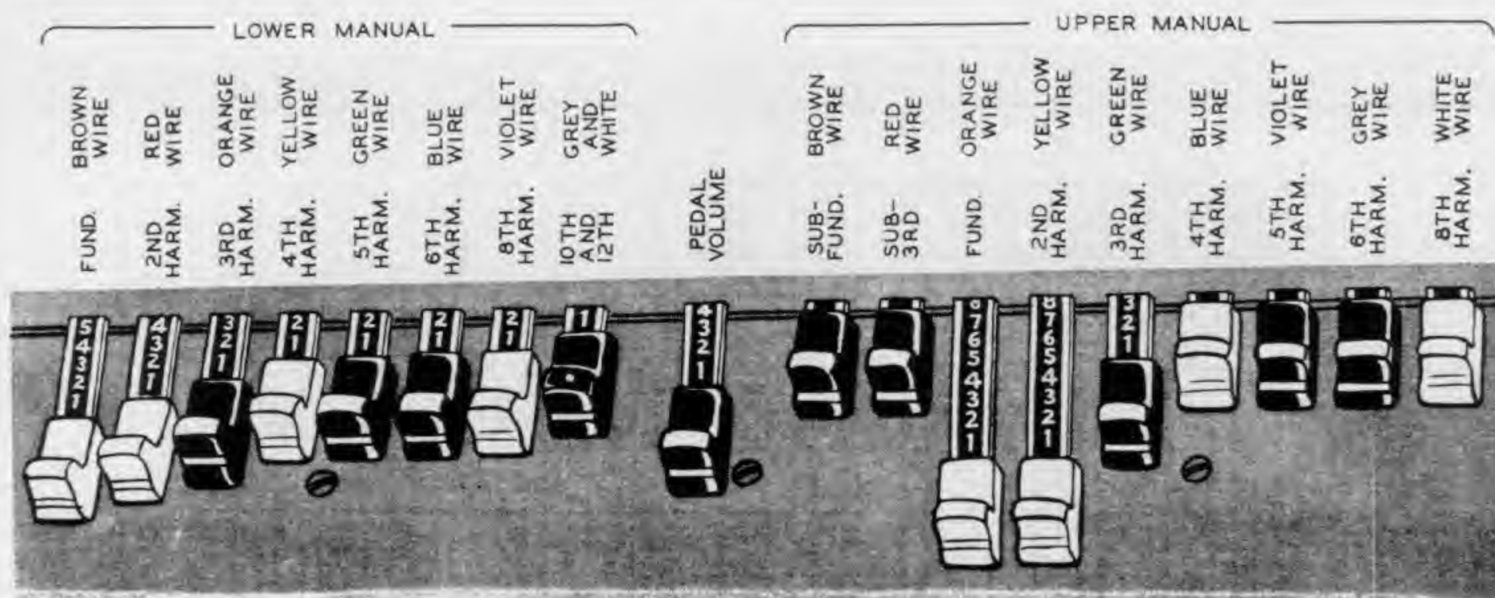
DRAWBAR ASSEMBLY
