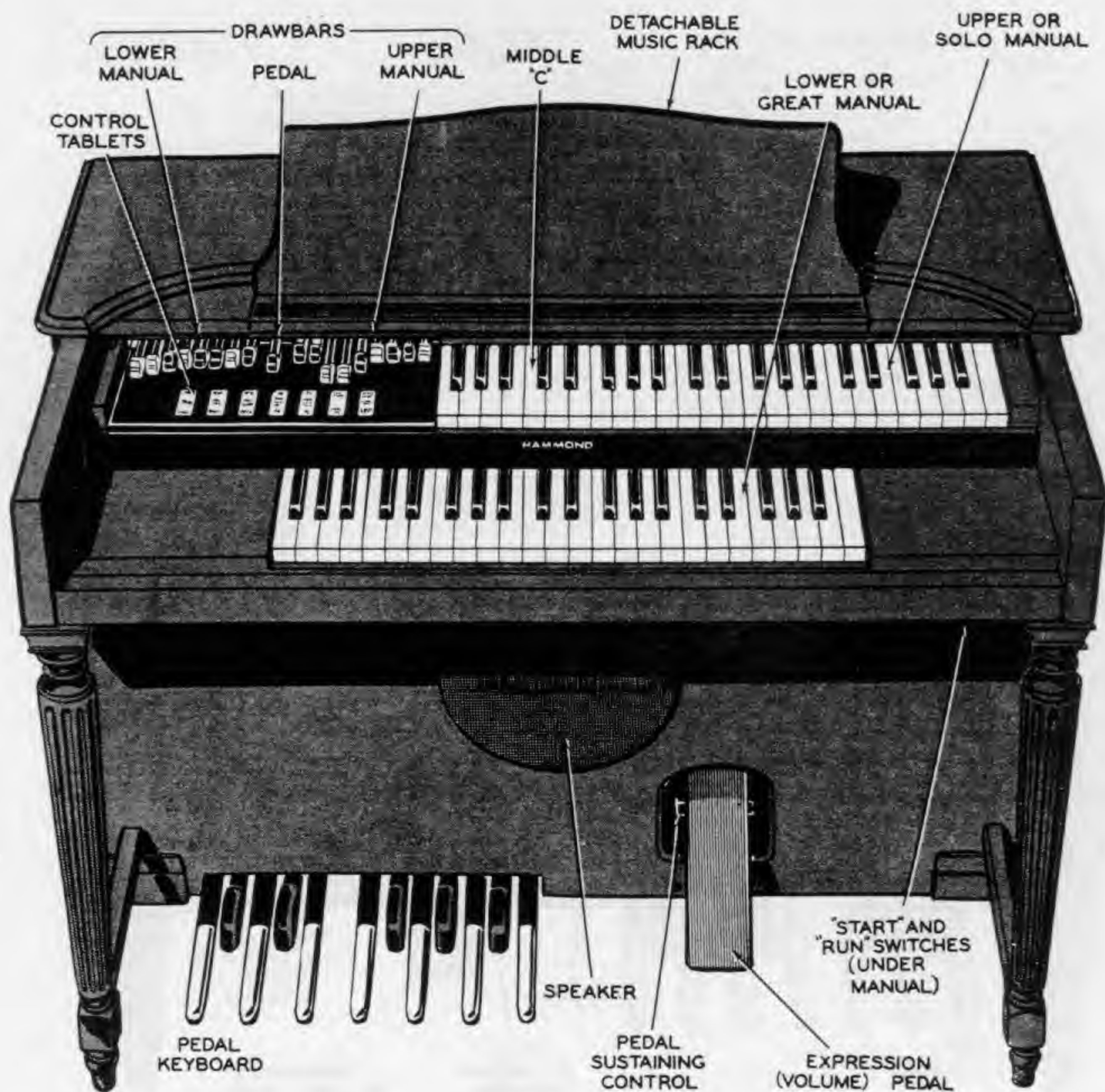
FRONT VIEW OF CONSOLE - MODEL M-2 ORGAN
