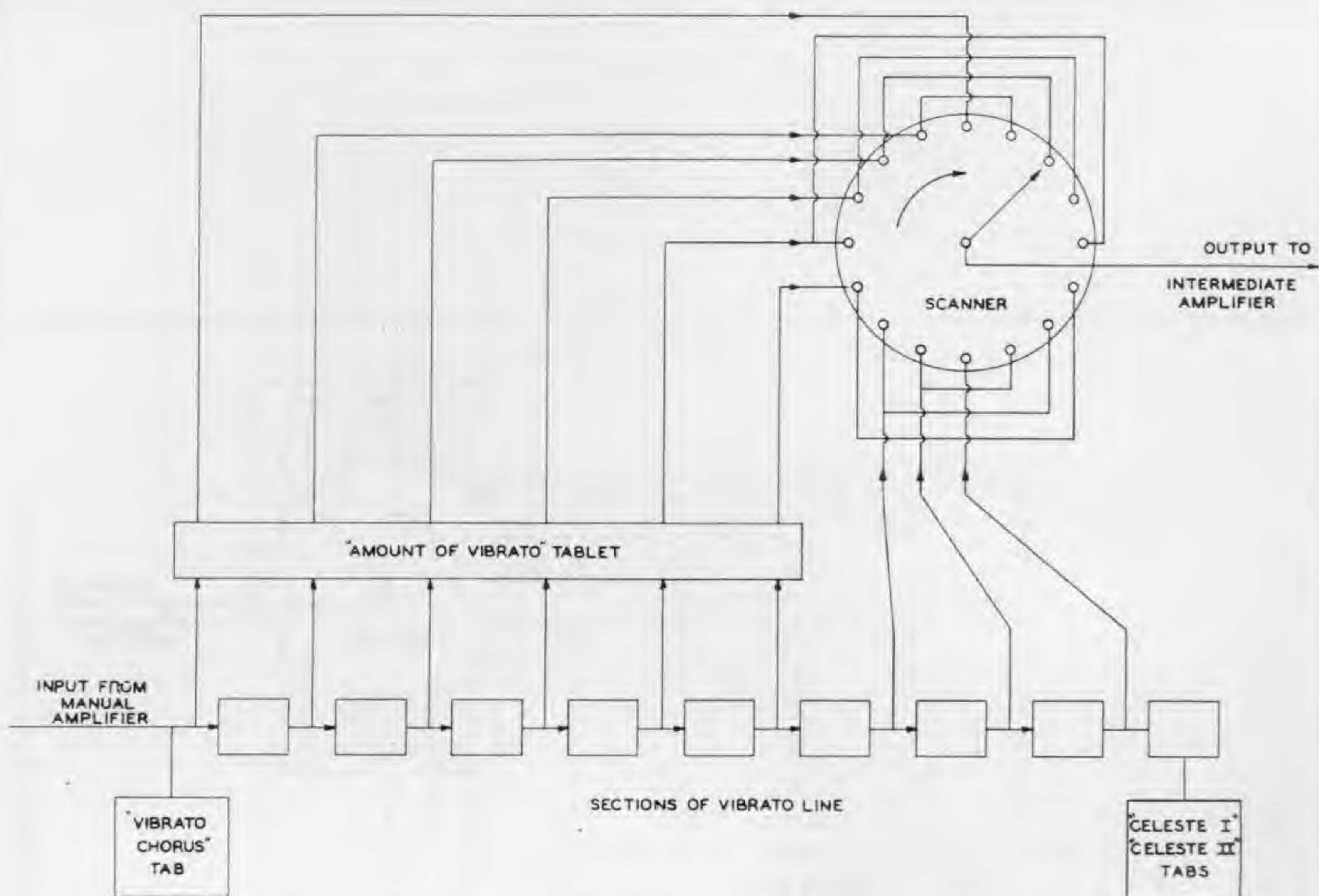
MODEL M-100 FUNDAMENTAL DIAGRAM OF VIBRATO SYSTEM
