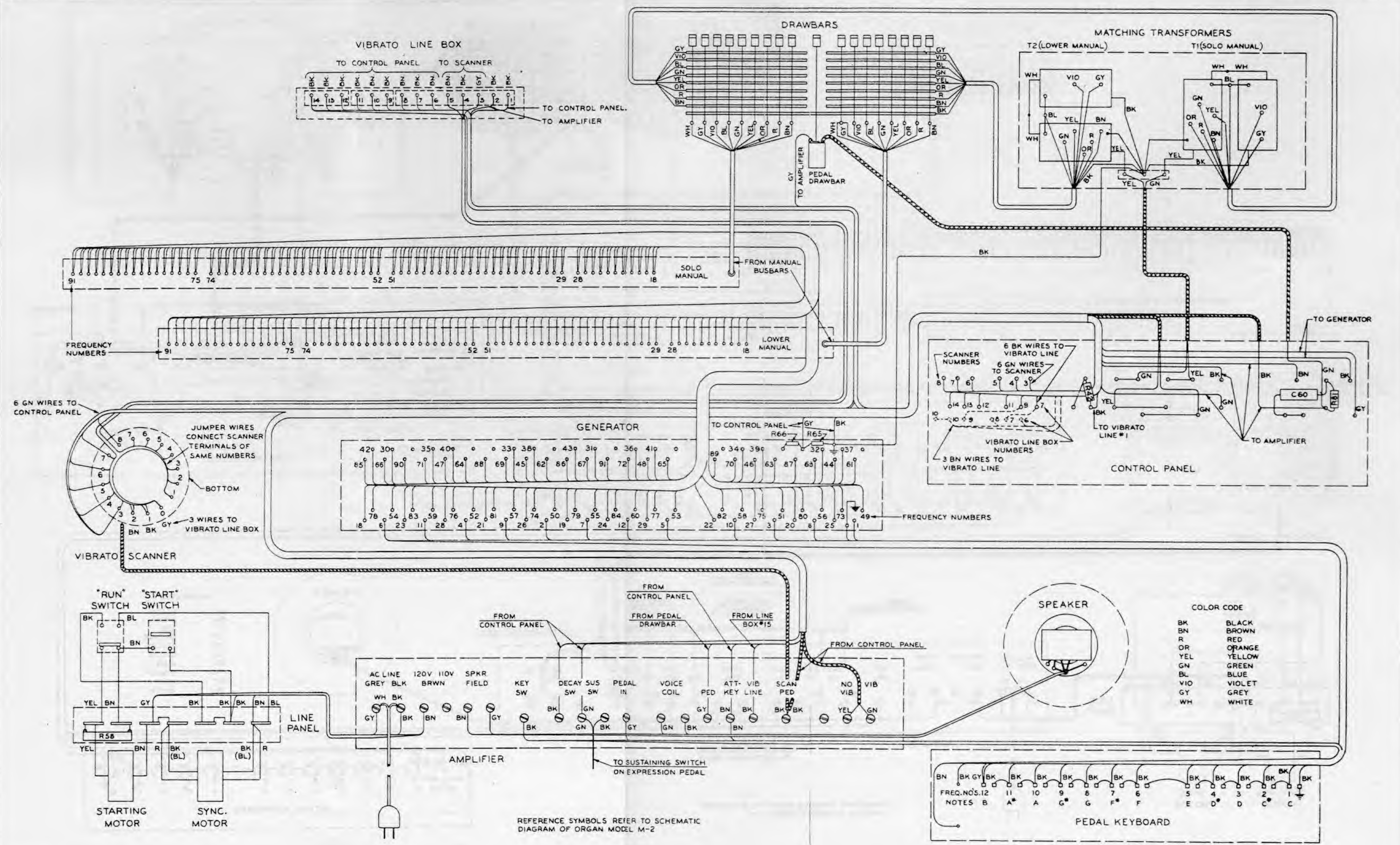
WIRING DIAGRAM MODEL M-2 - 25254 AND ABOVE FIGURE 43A
