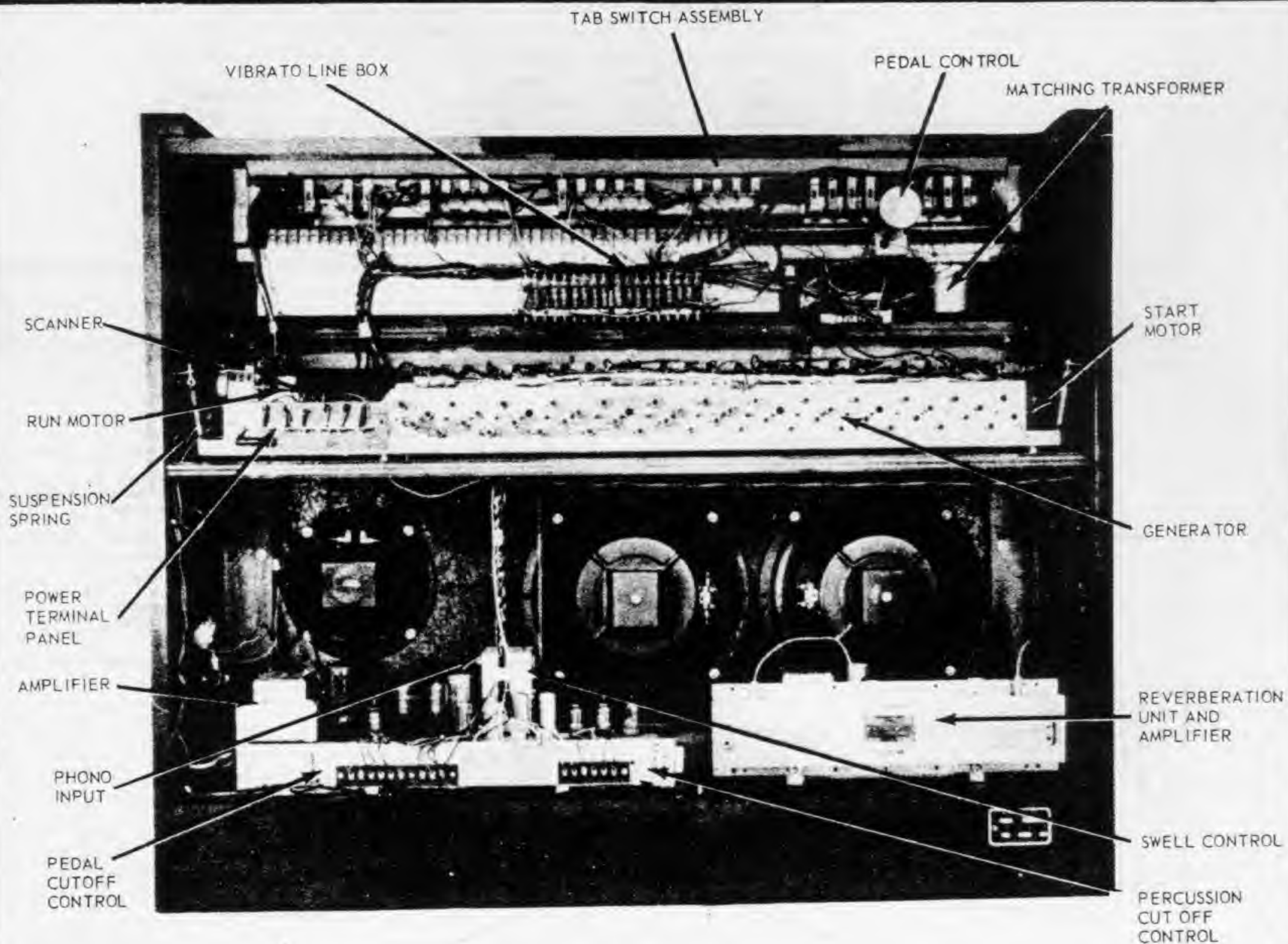
M-100 BACK VIEW OF CONSOLE GENERATOR DUST COVER REMOVED FIGURE 7
