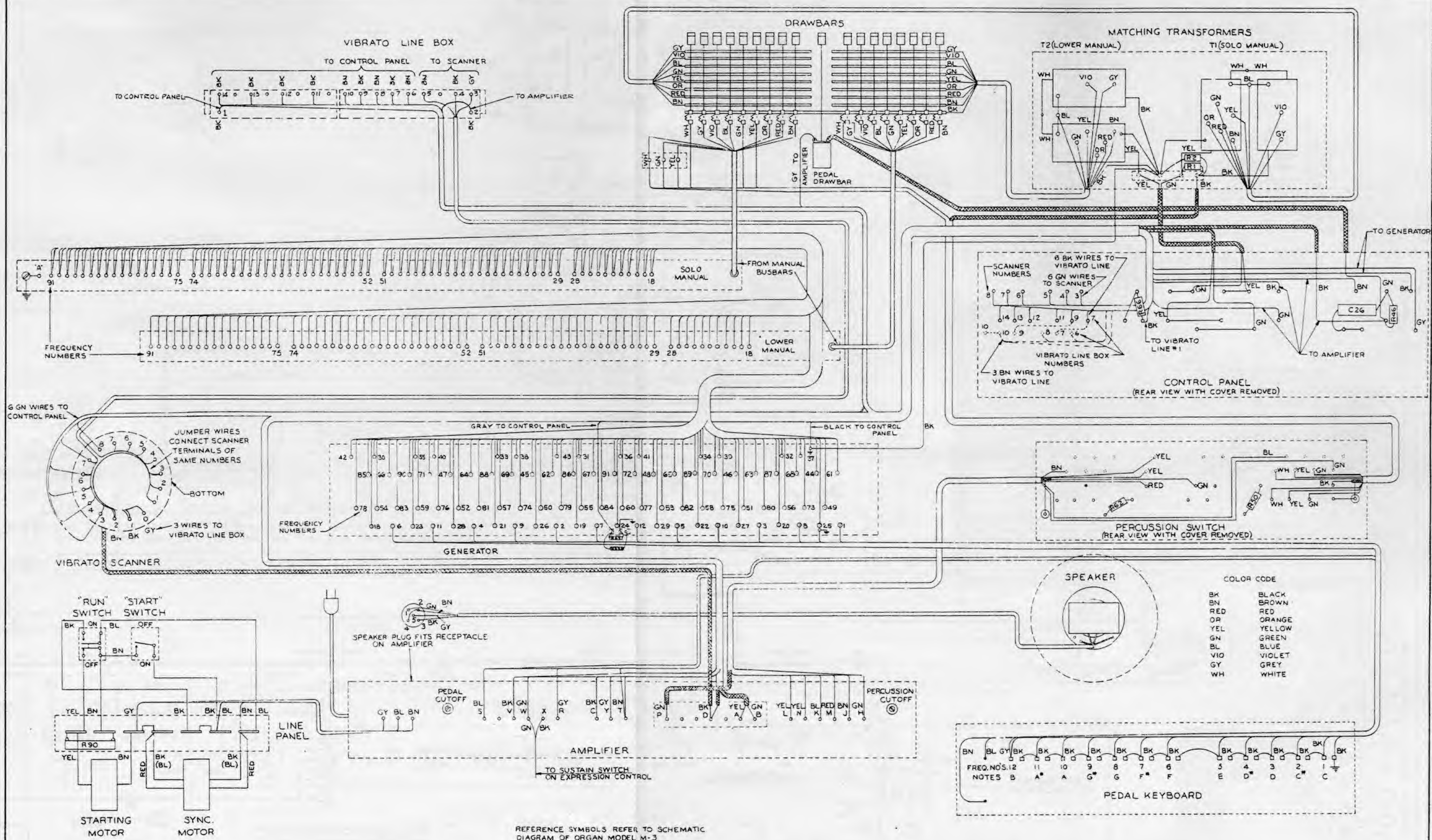
WIRING DIAGRAM MODEL M-3 - 90485 AND ABOVE FIGURE 45A
