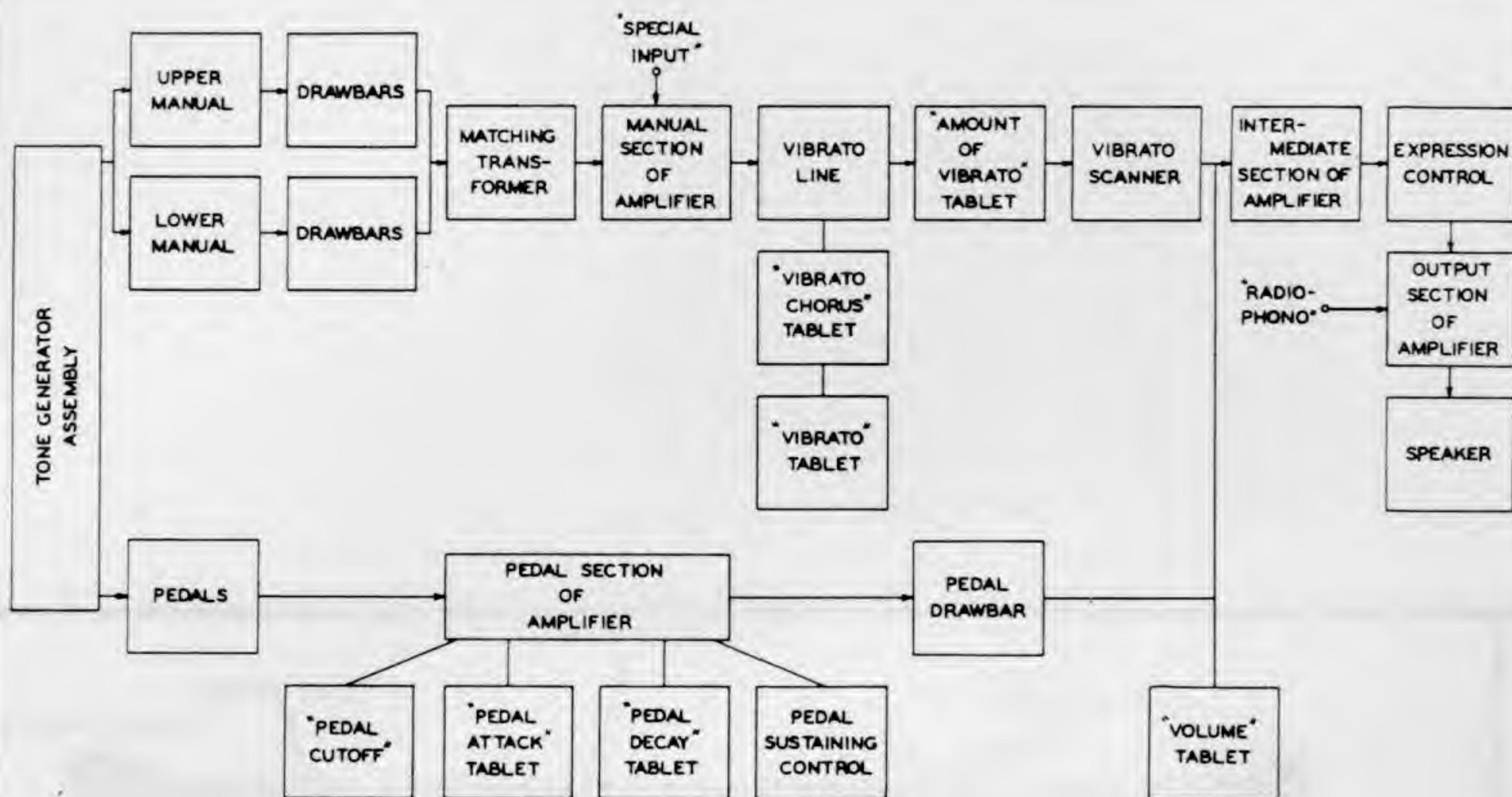
FIGURE 8 BLOCK DIAGRAM - MODEL M ORGAN
