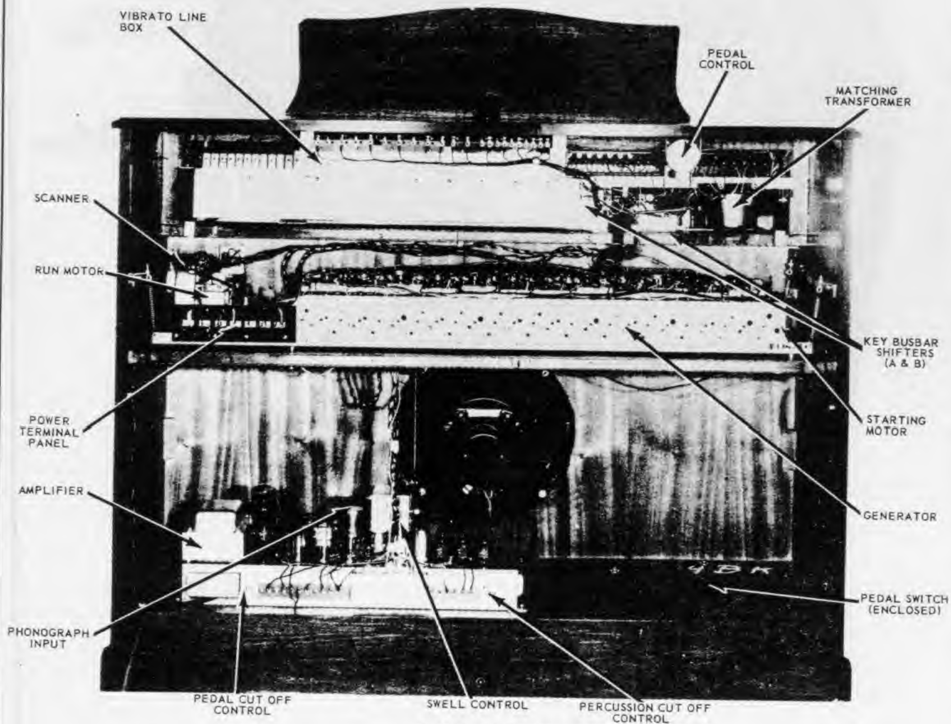
BACK VIEW OF CONSOLE M-3 (WITH DUST COVER REMOVED)
