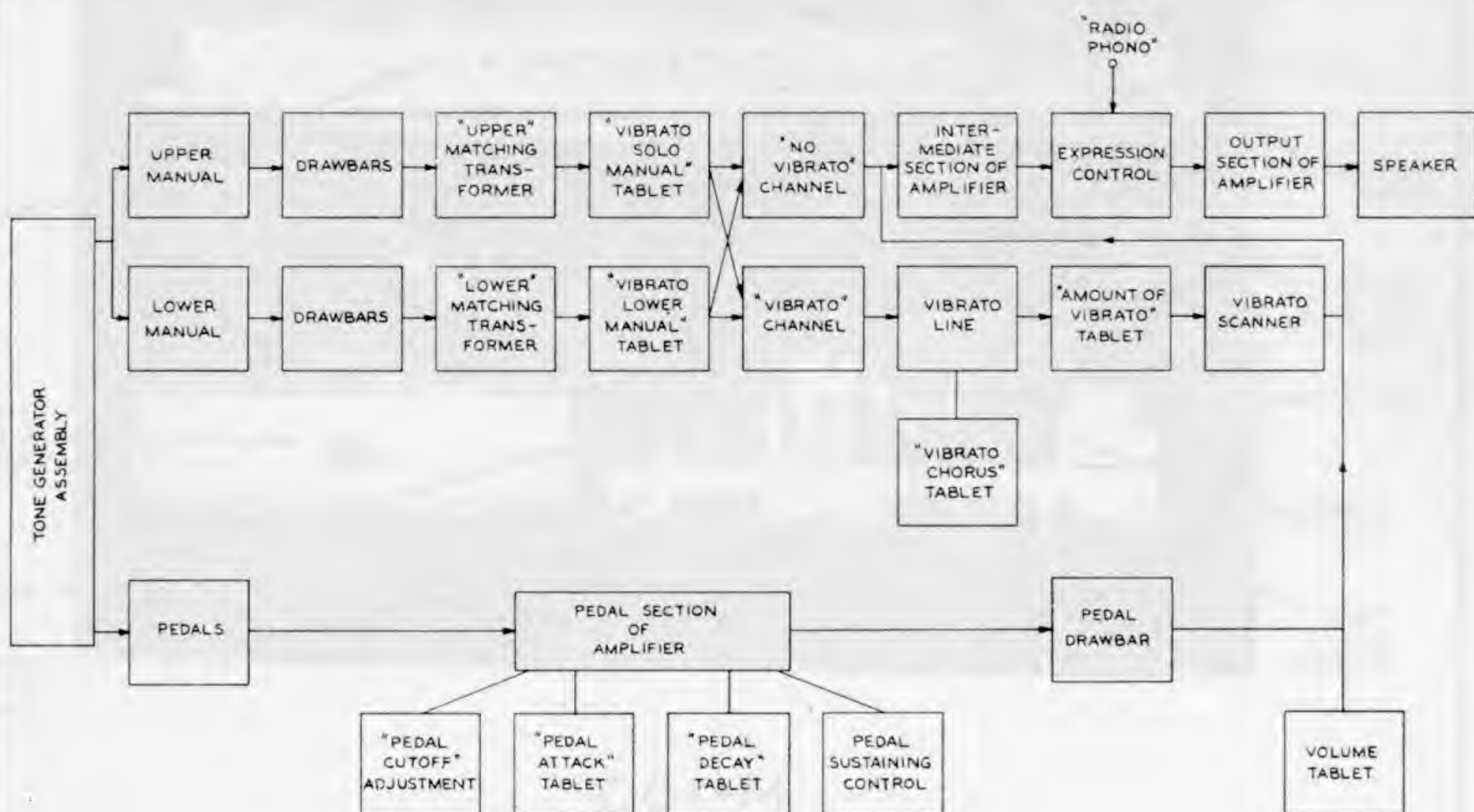
FIGURE 9 - BLOCK DIAGRAM - MODEL M-2
