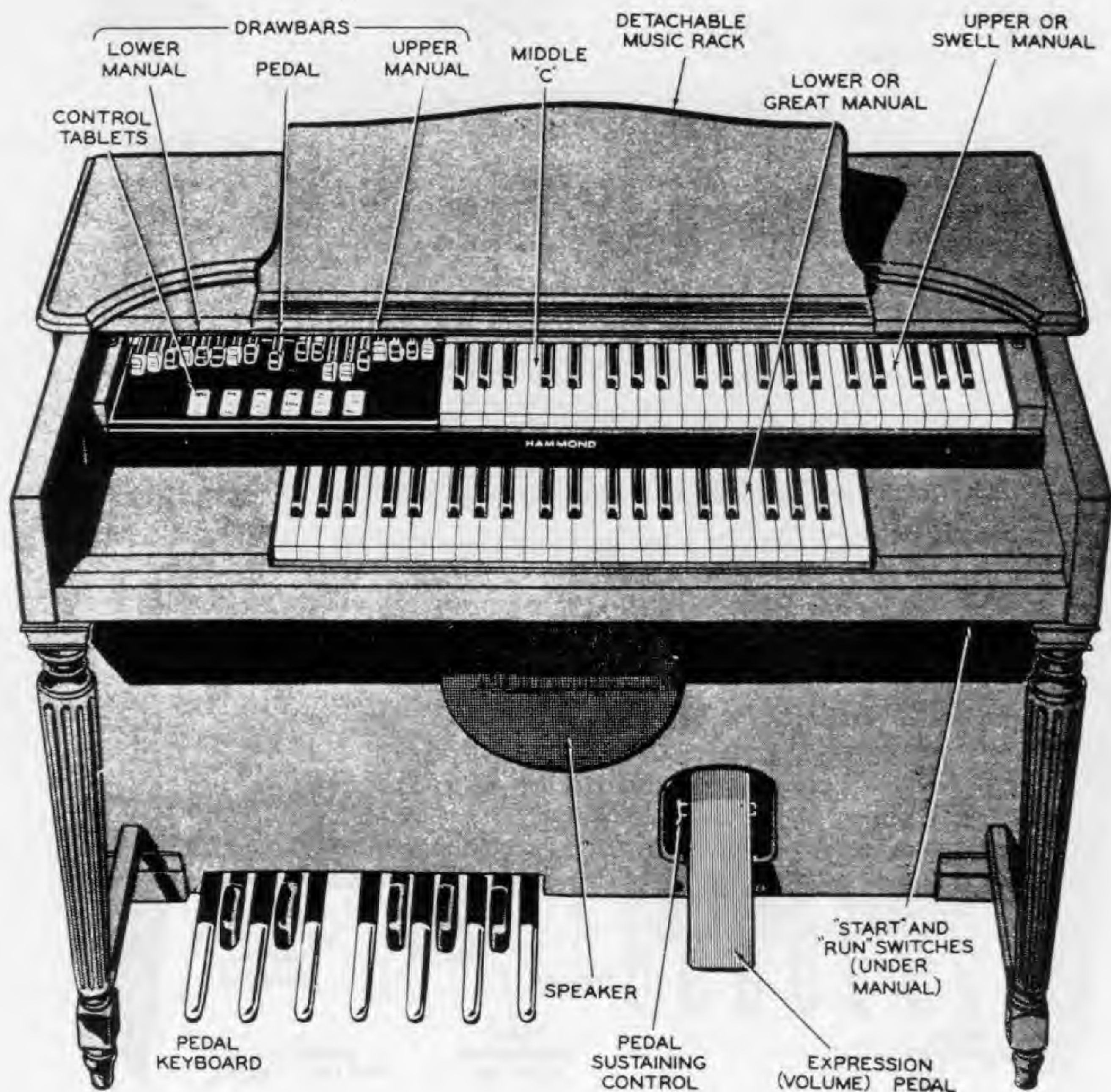
FRONT VIEW OF CONSOLE-MODEL M ORGAN
