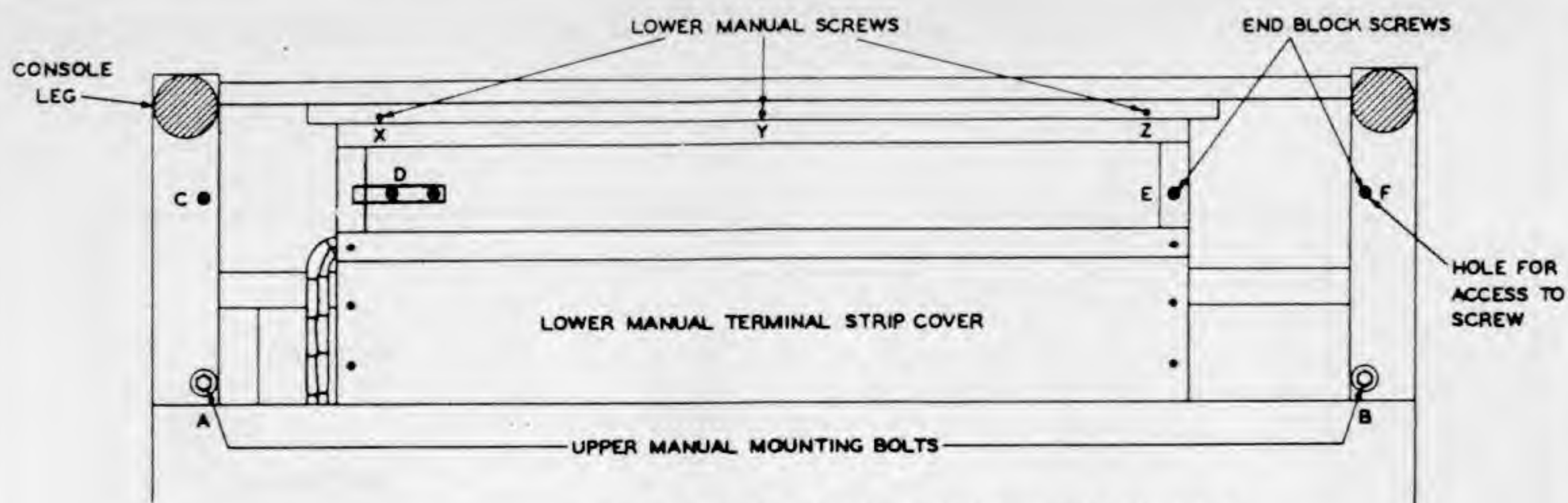
SCREWS HOLDING MANUALS (VIEW LOOKING UP UNDER KEYBOARD) FIGURE 33
