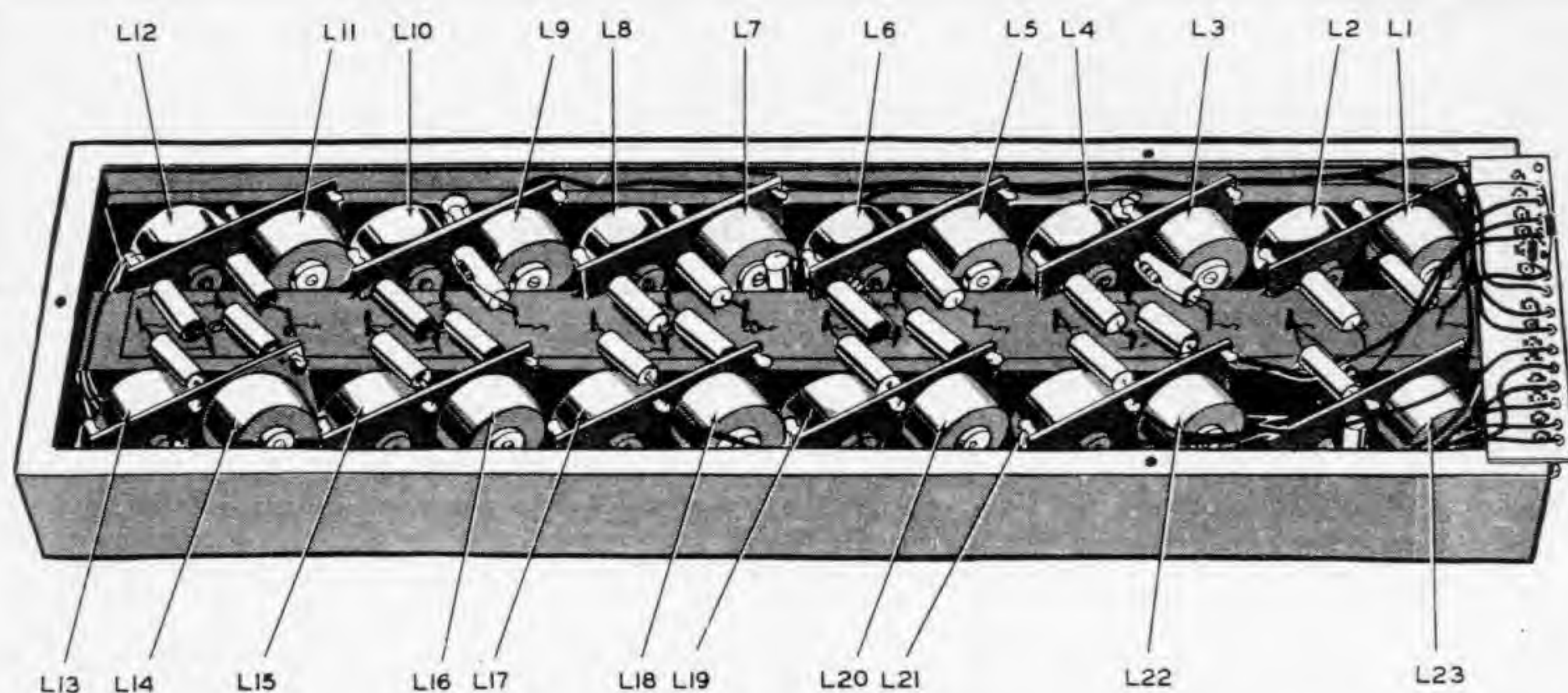
FIGURE 27 -VIBRATO LINE BOX-MODEL M AND M-2 ORGAN
