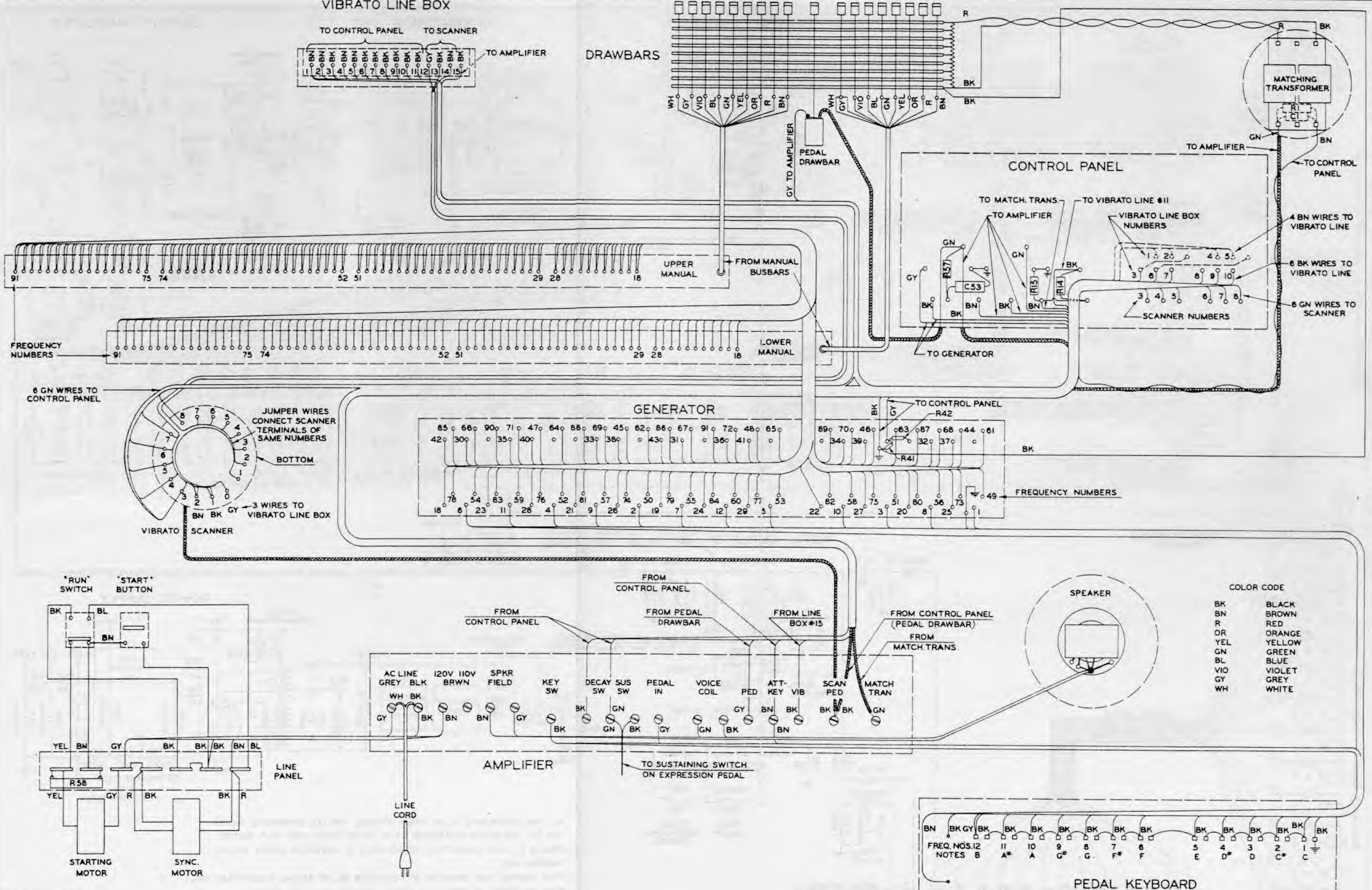
WIRING DIAGRAM MODEL M FIGURE 41
