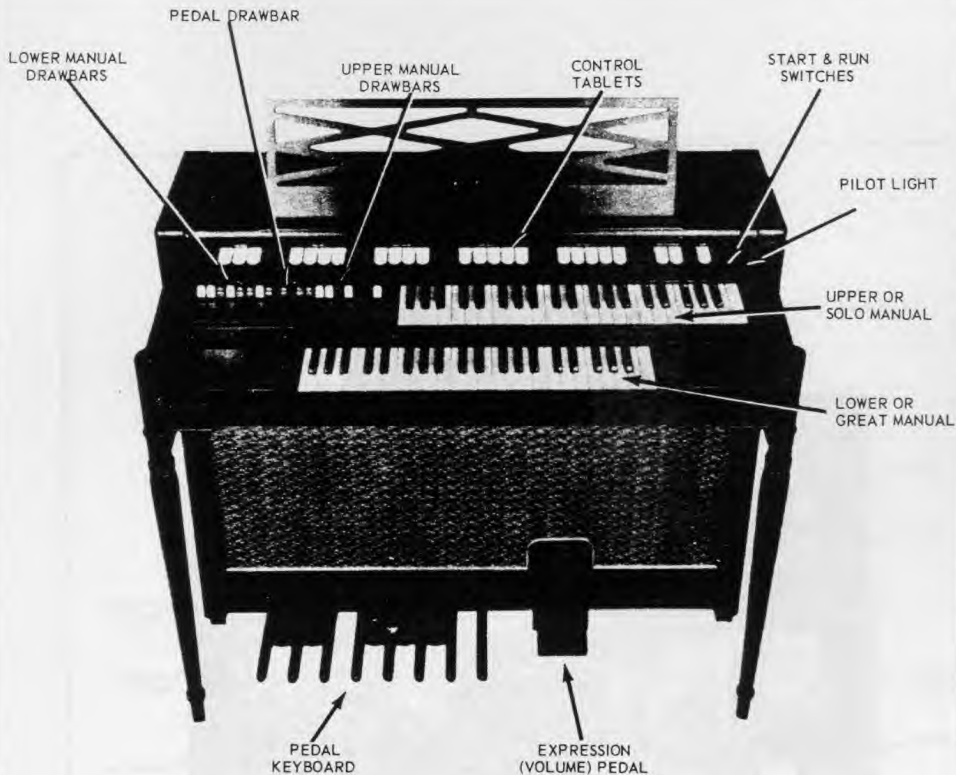
TYPICAL M-100 SERIES INSTRUMENT
