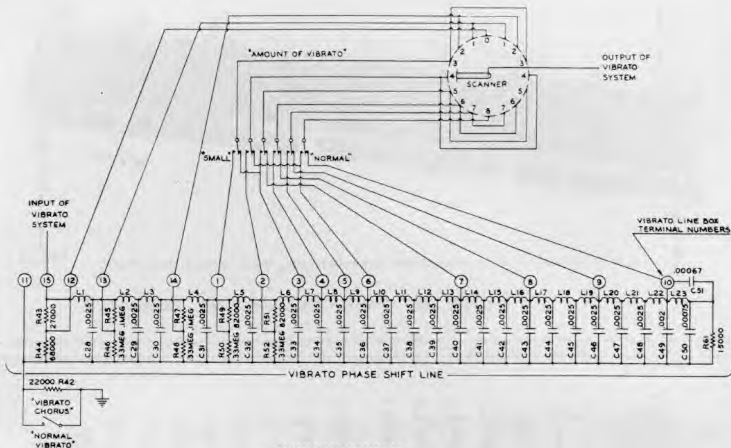
VIBRATO SYSTEM (MODEL M-2 CONSOLES SERIAL NUMBER 19000 TO 25253)
