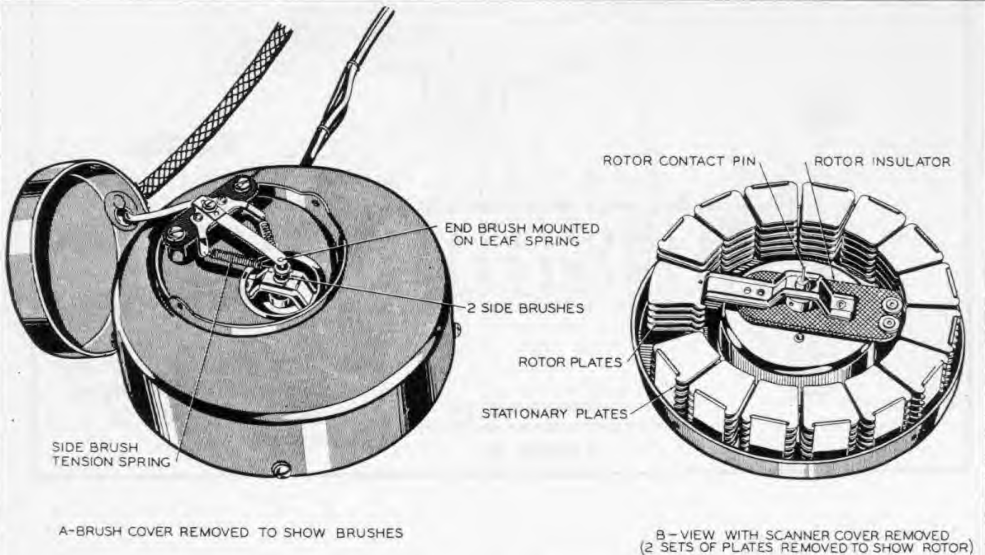
FIGURE 30 VIBRATO SCANNER
