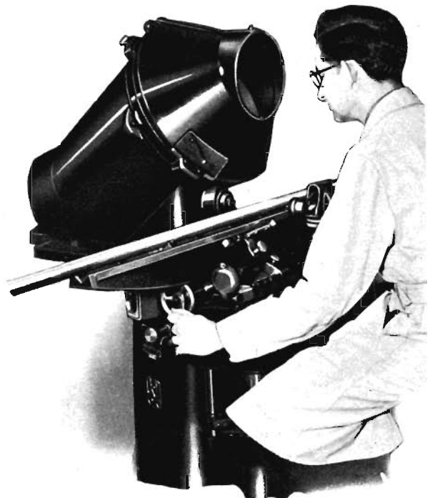
Fig. 1. Inspecting a Screw Thread with an Optical Comparator
