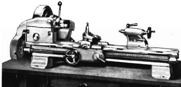
Model C South Bend Light Ten Bench Lathe
