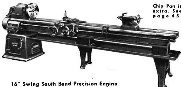
16" Swing South Bend Precision Engine Lathe with Center Leg
