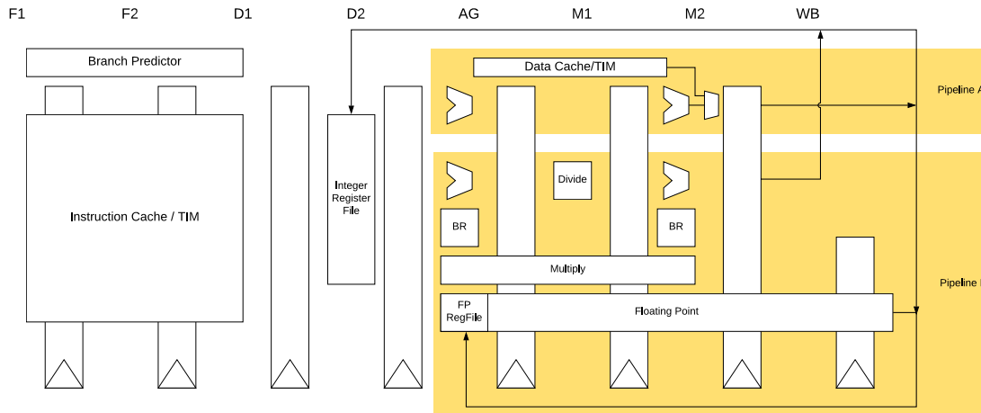
Figure 3: U74-MC Block Diagram
