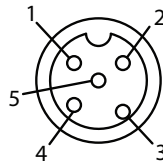
Figure 75 - Wiring Example for Alarm Inputs and Outputs
