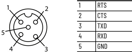
Figure 72 - Console Port Pinout
