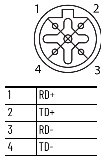
Figure 65 - 10/100 Connector Pinouts
