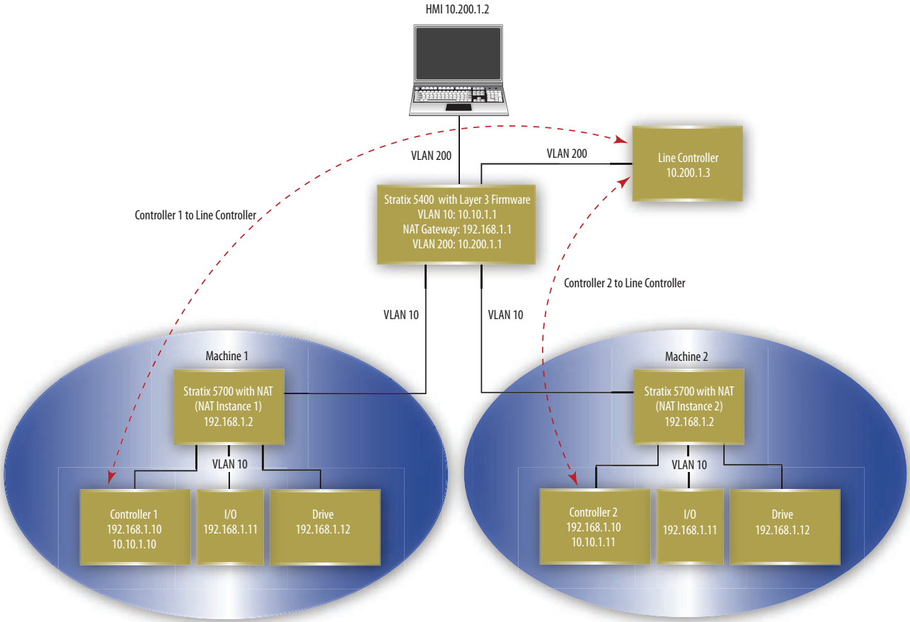
Figure 16 - Layer 3 Example with NAT in Stratix 5700 Switch
