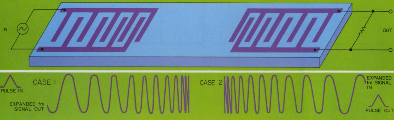
2. Surface-wave delay line with input and output transducers having graduated gratings that are mirror images of each other can be used as analog pulse expanders
