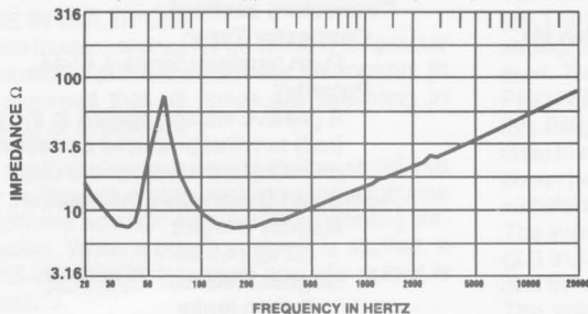
FIGURE 4 — Impedance in Typical Enclosure (4.0 ft³)
