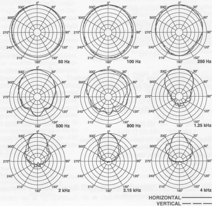
FIGURE 9 — Polar Response
