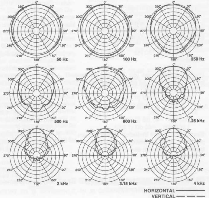
FIGURE 9 — Polar Response
