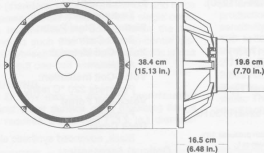
FIGURE 5 — Dimensions
