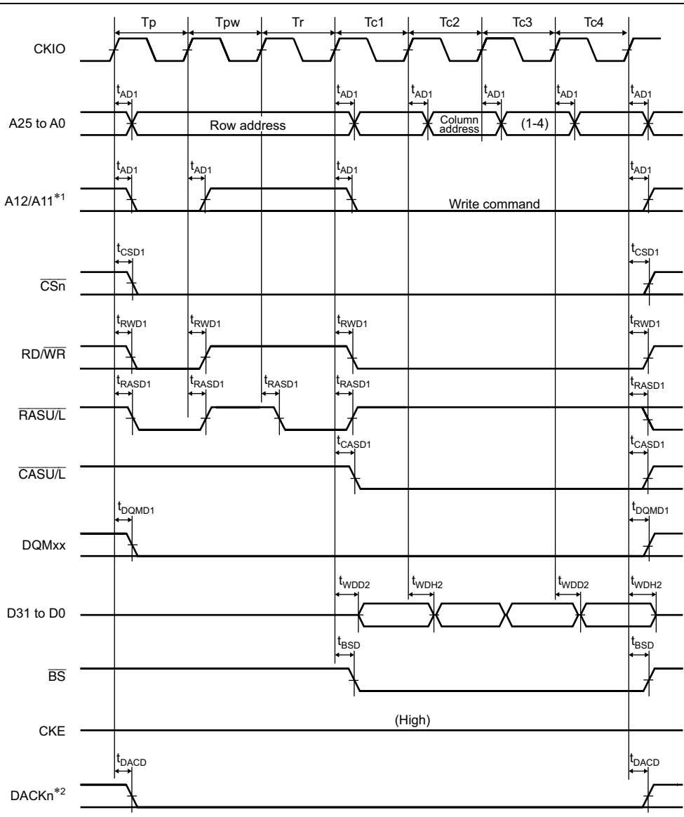
Figure 25.35 Synchronous DRAM Burst Write Bus Cycle (Single Write × 4) (Bank Active Mode: PRE + ACTV + WRITE Commands, Different Row Address, TRCD = 1 Cycle, TRWL = 1 Cycle)
