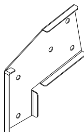
A100325 | SWING BEAM (1) | EXTENSION BRACKET-LEFT
