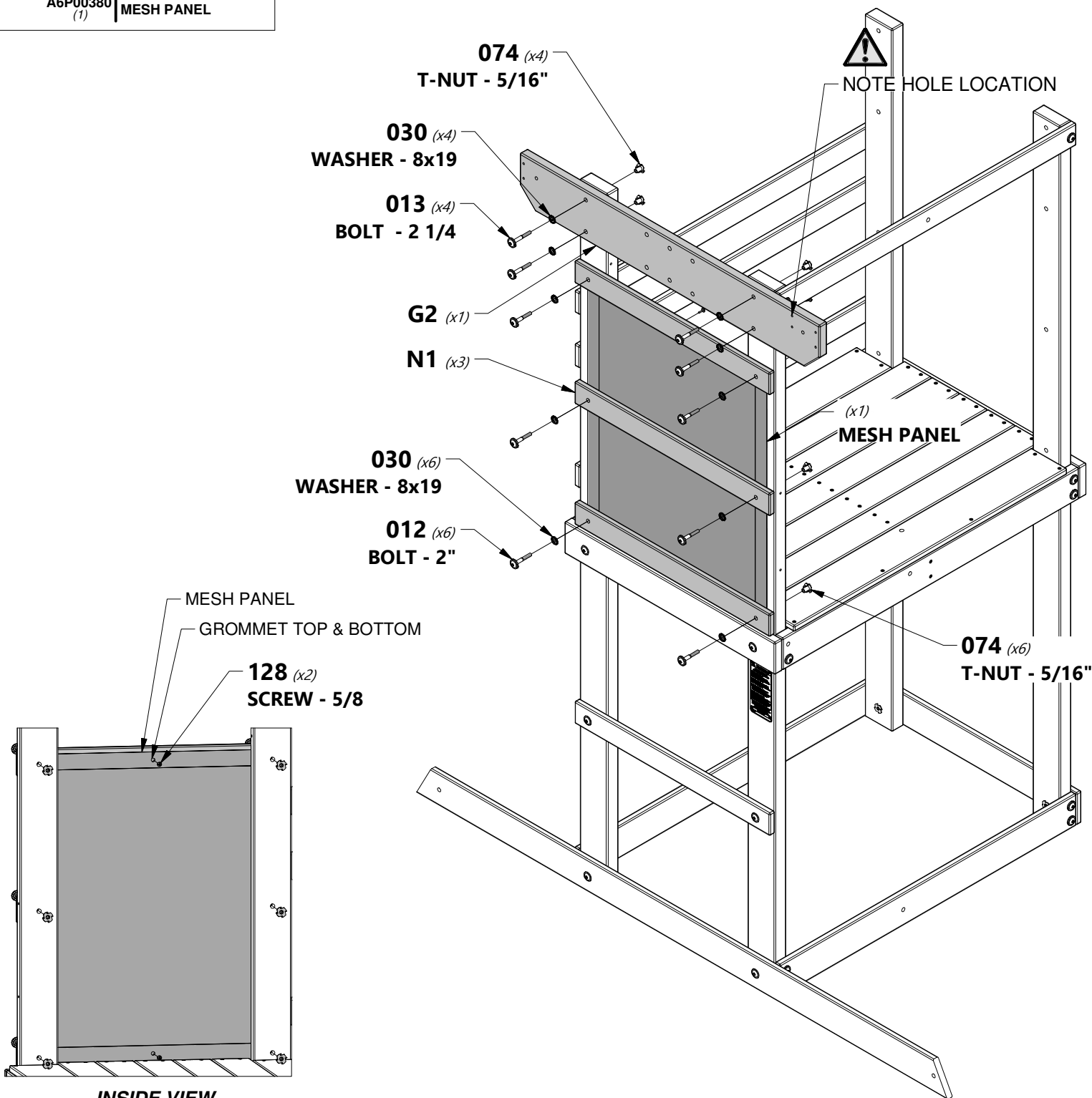
A6P00380 (1) MESH PANEL
