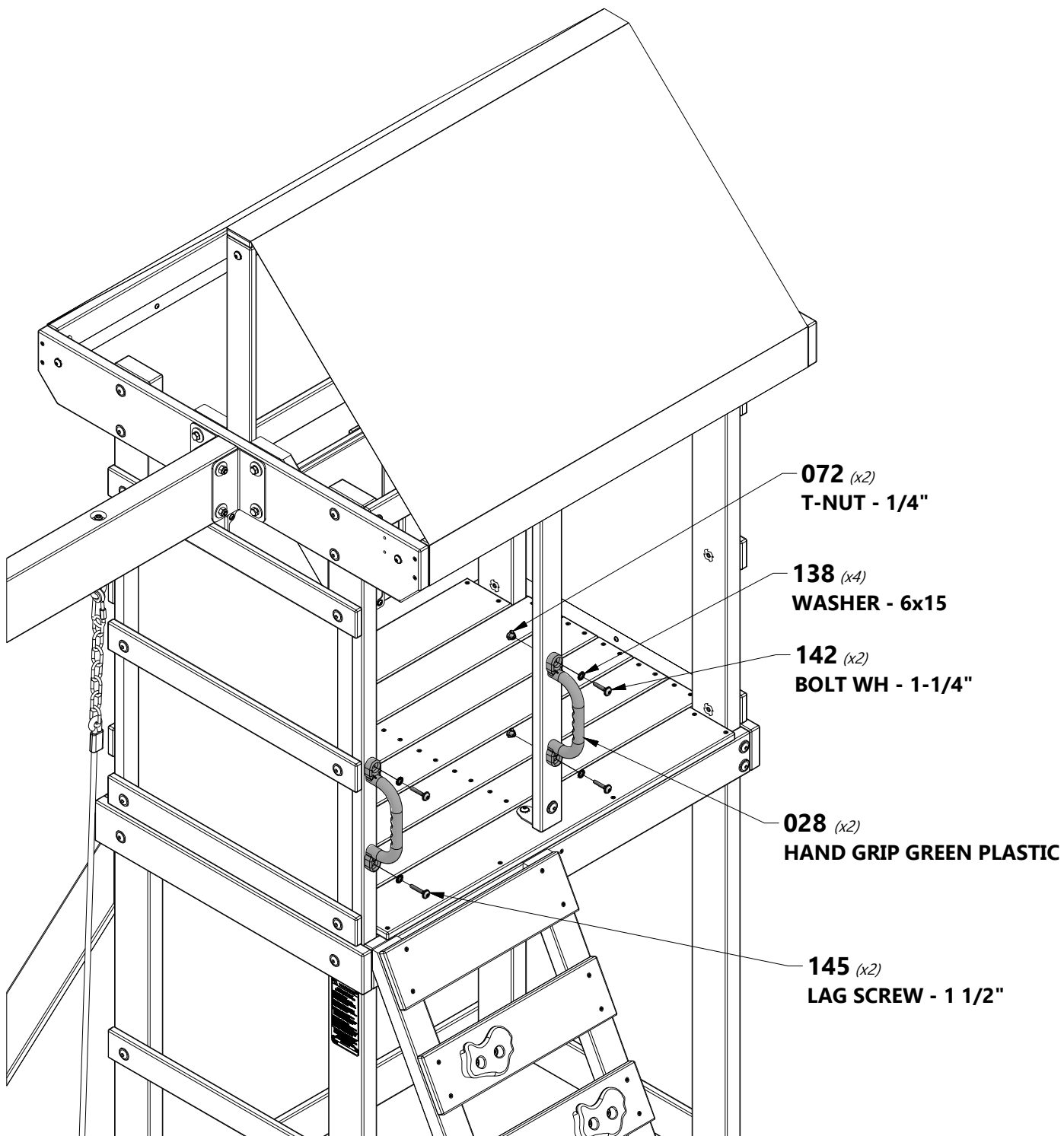
H100072 | T-NUT (2) | 1/4
